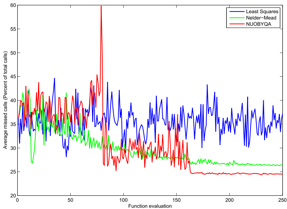
FIG 2. Results for three methods for tuning ADP coefficients in Edmonton, Canada. Each curve plots the estimated percentage of calls with response times above the threshold for 250 policies that are obtained within a tuning procedure.
