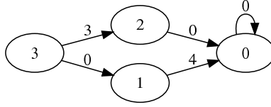
FIG 1. Example MDP.
