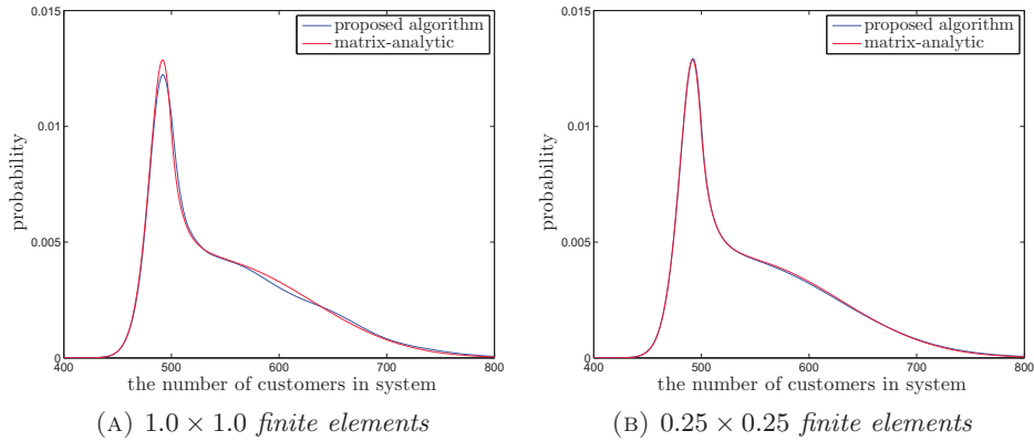
FIG 6: The stationary distribution of the customer number in the M/H_2/n + M queue, with \rho = 1.045 and n = 500 , computed (i) by the finite element algorithm using different meshes with the reference density in (3.21) and (3.23), and (ii) by the matrix-analytic method.
