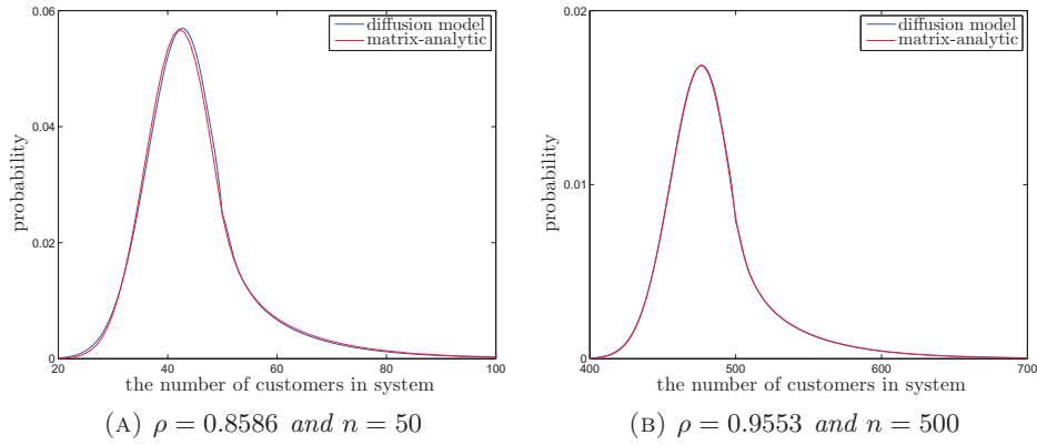
FIG 3: The stationary distribution of the customer number in the M/H_2/n queue, computed (i) by the finite element algorithm for the diffusion model with the reference density in (3.21) and (3.22), and (ii) by the matrix-analytic method.
