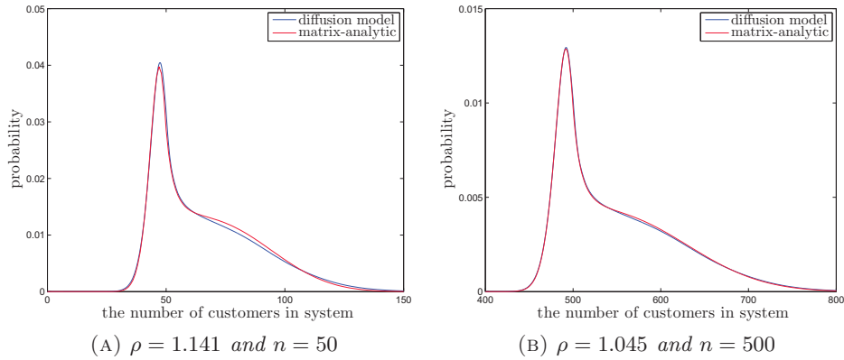
FIG 1: The stationary distribution of the customer number in the M/H_2/n + M queue, computed (i) by the finite element algorithm for the diffusion model with the reference density in (3.21) and (3.23), and (ii) by the matrix-analytic method.
