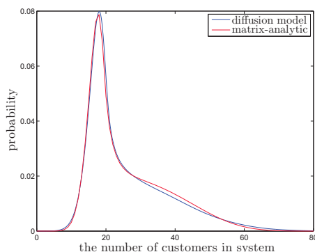
FIG 2: The stationary distribution of the customer number in the M/H_2/n+M queue, with \rho = 1.112 and n = 20 , computed (i) by the finite element algorithm for the diffusion model with the reference density in (3.21) and (3.23), and (ii) by the matrix-analytic method.
