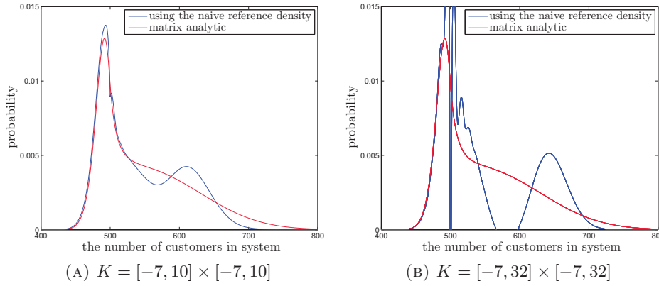
FIG 5: The stationary distribution of the customer number in the M/H_2/n + M queue, with \rho = 1.045 and n = 500 , computed (i) by the finite element algorithm with the “naive” reference density, and (ii) by the matrix-analytic method.
