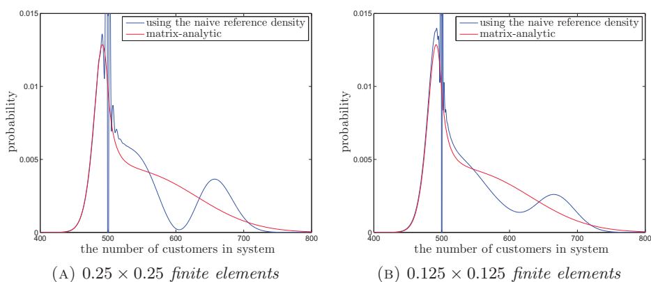
FIG 7: The stationary distribution of the customer number in the M/H_2/n + M queue, with \rho = 1.045 and n = 500 , computed (i) by the finite element algorithm using the “naive” reference density and different meshes, and (ii) by the matrix-analytic method.
