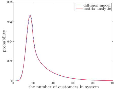
FIG 4: The stationary distribution of the customer number in the M/H_2/n queue, with \rho = 0.8882 and n = 20 , computed (i) by the finite element algorithm for the diffusion model with the reference density in (3.21) and (3.22), and (ii) by the matrix-analytic method.
