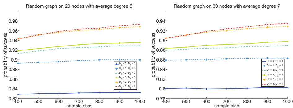
FIG 3. Plots of the probability of success versus the sample size for random graphs with D_1 = 0, \dots, 3 and D_2 = 0, 1 .
