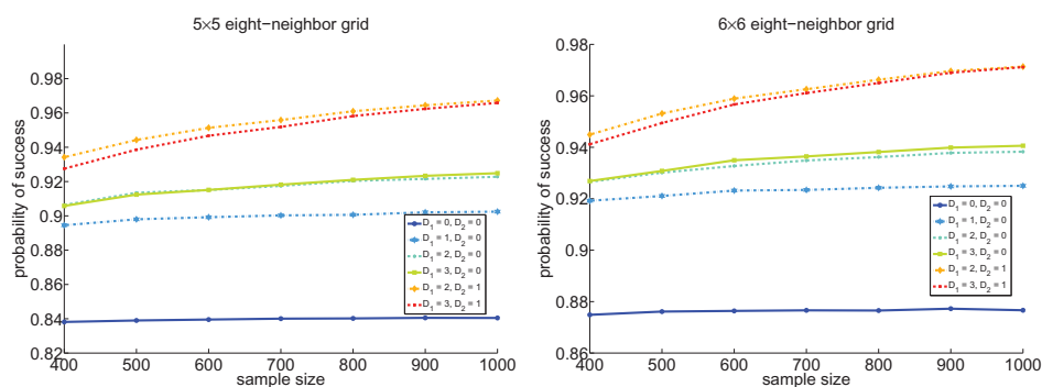
FIG 2. Plots of the probability of success versus the sample size for 5 \times 5 and 6 \times 6 eight-neighbor grids with D_1 = 0, \dots, 3 and D_2 = 0, 1 .
