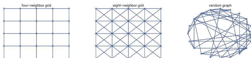
FIG 1. Illustrations of four-neighbor grid, eight-neighbor grid and the random graph.
