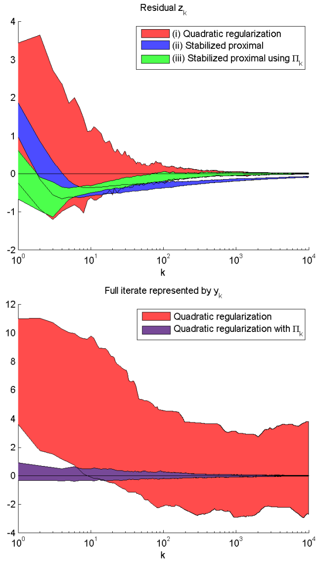
FIG 3. Convergence of residual for proximal iteration using quadratic regularization in Example 15, compared with stabilized proximal iterations. The top figure shows the residuals z_k of the quadratic regularization algorithm [iteration (i)], compared with those of proximal iterations [(ii) and (iii)] that use stabilization instead. The bottom figure shows the y_k -portion of the iterates x_k generated by iteration (i), and the y_k -portion of the iterates \hat{x}_k = \Pi_k x_k . It can be seen that \{x_k\} is divergent, while \{\hat{x}_k\} is convergent.
