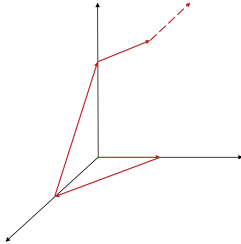
FIG 1. An optimal path with five pieces.
