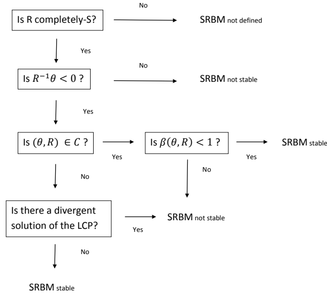
FIG 2. Existence and stability of SRBM in the octant.
