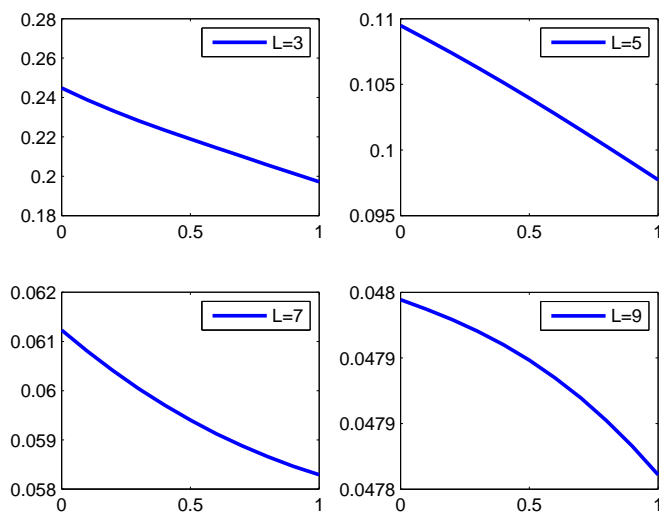
FIG 2. For \lambda = 0.99 , the marginal value of sampling V(L, L + q) with increasing q from 0 to 1 and varying L .
