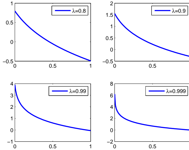
FIG 4. The natural logarithm of V(1, 1 + q) with increasing q from 0 to 1, for varying arrival rate \lambda .
