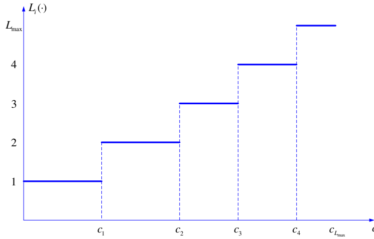
FIG 5. The best response strategy L_i(\cdot) \in BR(L_{-i}(\cdot)) is a non-decreasing step function. The jumping points are denoted by 0 = c_0 < c_1 < \dots < c_{L_{\max}} = c_{\max} .
