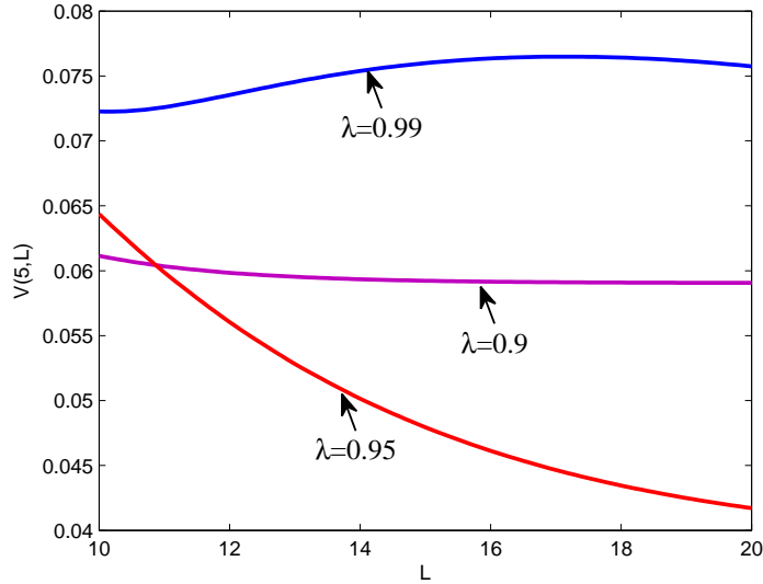
FIG 1. The marginal value of sampling V(5, L) with increasing L from 10 to 20 and varying arrival rate \lambda .
