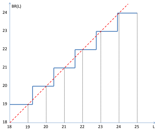
FIG 3. The best response with respect to L for \lambda = 0.999 and \frac{c_s}{c} = 0.0148 .
