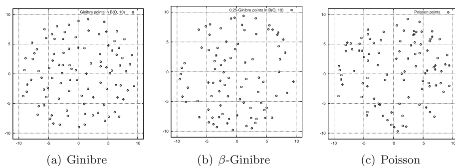
FIG 1. Realizations of the Ginibre process, the \beta -Ginibre process with \beta = 0.25 and the homogeneous Poisson process of intensity 1/\pi within the ball b(O, 10) .
