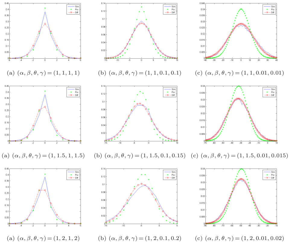
FIG 5. Density functions by simulation method, Poisson approximation, and heavy traffic diffusion approximation, when inter-arrival times follow hyper-exponential distribution.
