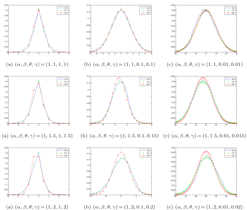
FIG 2. Density functions by simulation method, Poisson approximation, and heavy traffic diffusion approximation, when inter-arrival times follow exponential distribution.
