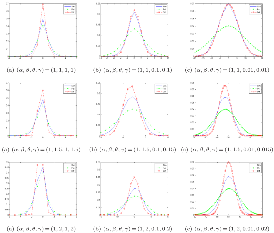
FIG 3. Density functions by simulation method, Poisson approximation, and heavy traffic diffusion approximation, when inter-arrival times follow uniform distribution.
