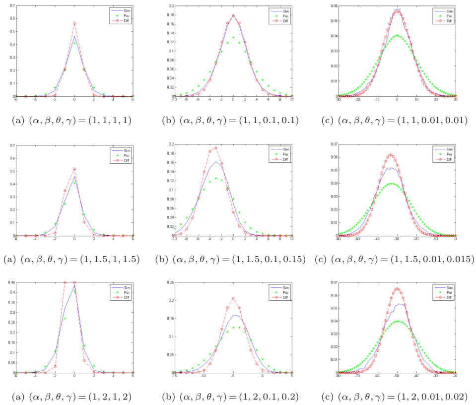
FIG 4. Density functions by simulation method, Poisson approximation, and heavy traffic diffusion approximation, when inter-arrival times follow Erlang distribution.
