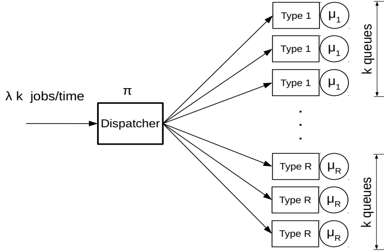
FIG 1. Structure of the parallel queueing model under investigation.
