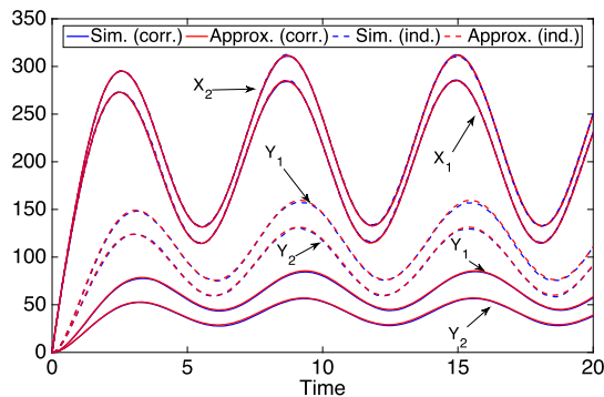
FIG 2. Comparison of fluid approximations with simulations when the service times have the Marshall-Olkin bivariate exponential distributions with correlation \rho = 0 and \rho = 0.5 . The figure shows the simulated values of X_i and Y_i , i = 1, 2 , and their corresponding fluid approximations (solid lines for \rho = 0.5 and dashed lines for \rho = 0 ). The values for the X_i are the same when \rho = 0 and \rho = 0.5 , while the values of Y_i when \rho = 0.5 are smaller than those when \rho = 0 .
