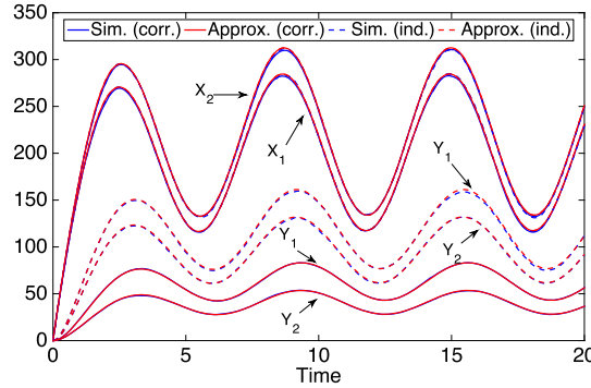
FIG 3. Comparison of fluid approximations with simulations when the service times have the Marshall-Olkin bivariate hyperexponential distributions with correlation \rho = 0 and \rho = 0.5 (solid lines for \rho = 0.5 and dashed lines for \rho = 0 ). The figure shows the simulated values of X_i and Y_i , i = 1, 2 , and their corresponding fluid approximations. The same observations can be made as in Figure 2.
