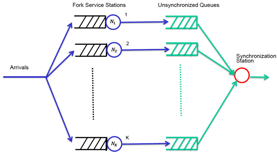
FIG 1. A fundamental fork-join network with finite servers.
