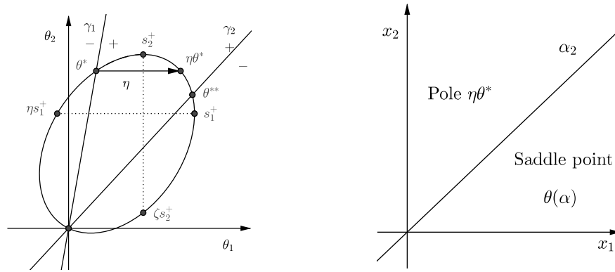
FIG 23. Theorem 26 case (iib)
