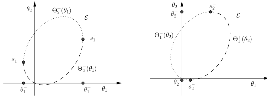
FIG 5. Functions \Theta_2^\pm(\theta_1) and \Theta_1^\pm(\theta_2) on [\theta_1^-, \theta_1^+] and [\theta_2^-, \theta_2^+]
