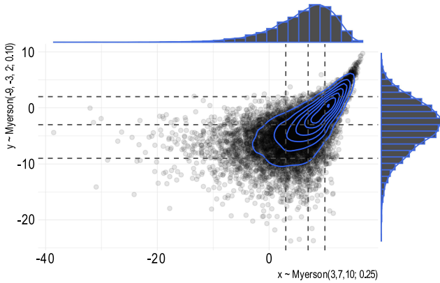
Figure 10. (Color online) Samples from the Bivariate Myerson Distribution Joined by the Joe Copula ( \theta = 3 )
