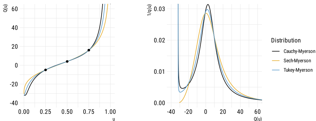
Figure 4. (Color online) Quantile Function and Quantile Density of Generalized Myerson Distributions with Unreliable Kernels
