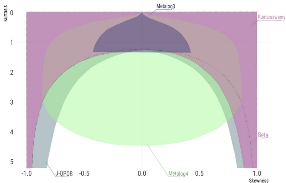
Figure 7. (Color online) Robust Skewness vs. Robust Kurtosis for Some Bounded Distributions
