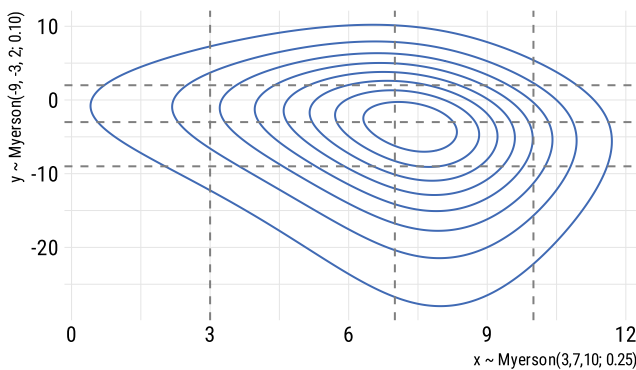
Figure 9. (Color online) Density of Generalized Myerson Distributions Joined by Type II Bivariate Logistic Distribution
