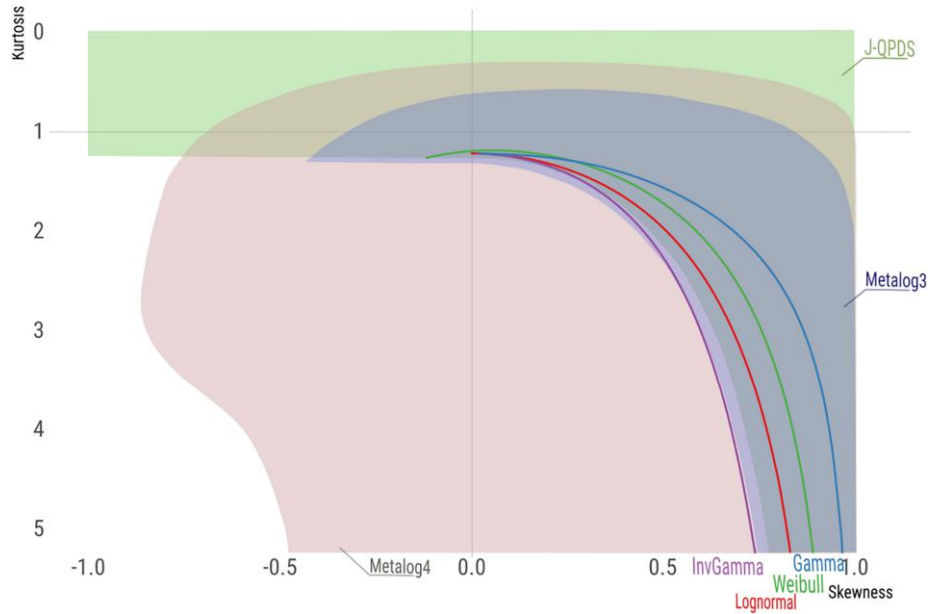
Figure 6. (Color online) Robust Skewness vs. Robust Kurtosis for Some Left-Bounded Distributions
