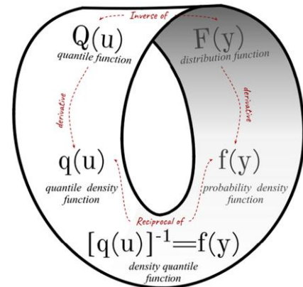
Figure 1. (Color online) Möbius Strip of Probability Functions (Perepolkin et al. 2023)
