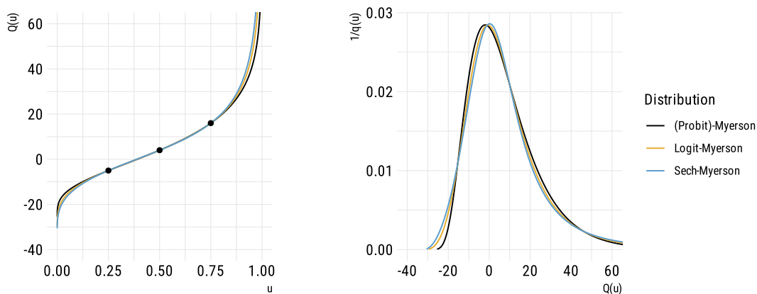
Figure 3. (Color online) Quantile Function and Quantile Density of Generalized Myerson Distributions
