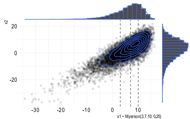
Figure 11. (Color online) Samples from the Bivariate Myerson Quantile Function
