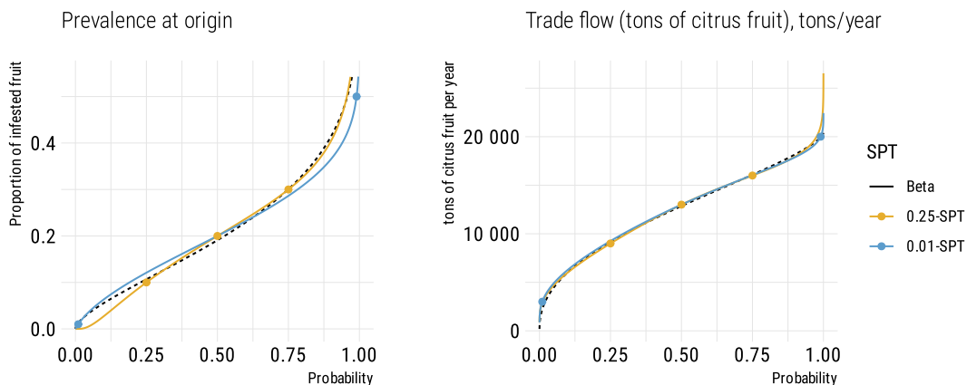
Figure 2. (Color online) Fitted J-QPD-B (Left) and J-QPD-S (Right) Distribution for Prevalence at Origin and Total Trade Flow, Respectively
