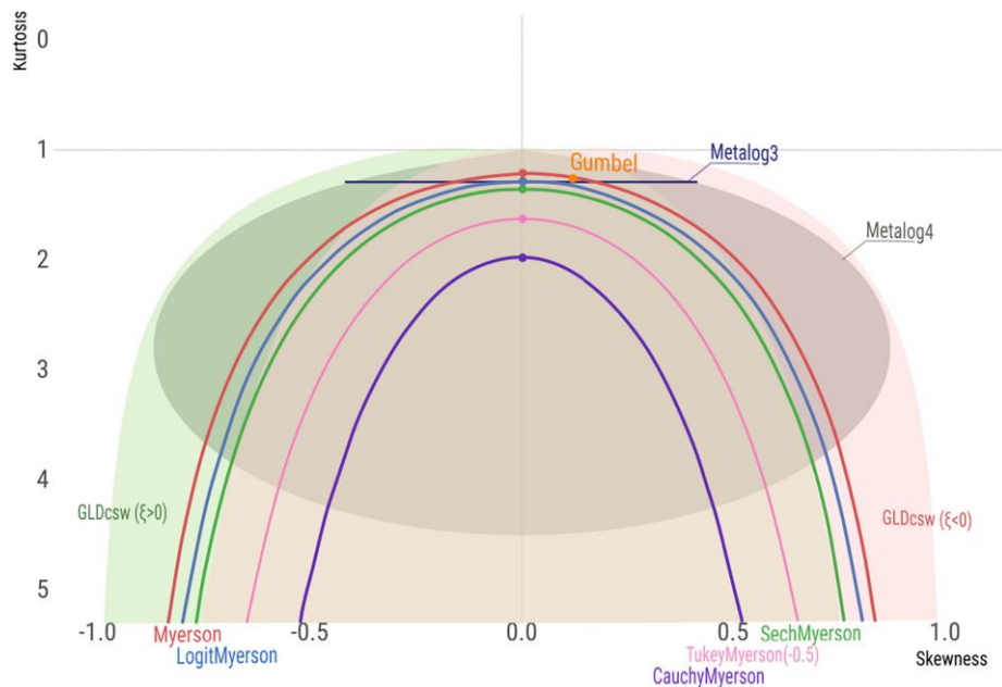
Figure 5. (Color online) Robust Skewness vs. Robust Kurtosis for Some Unbounded Distributions
