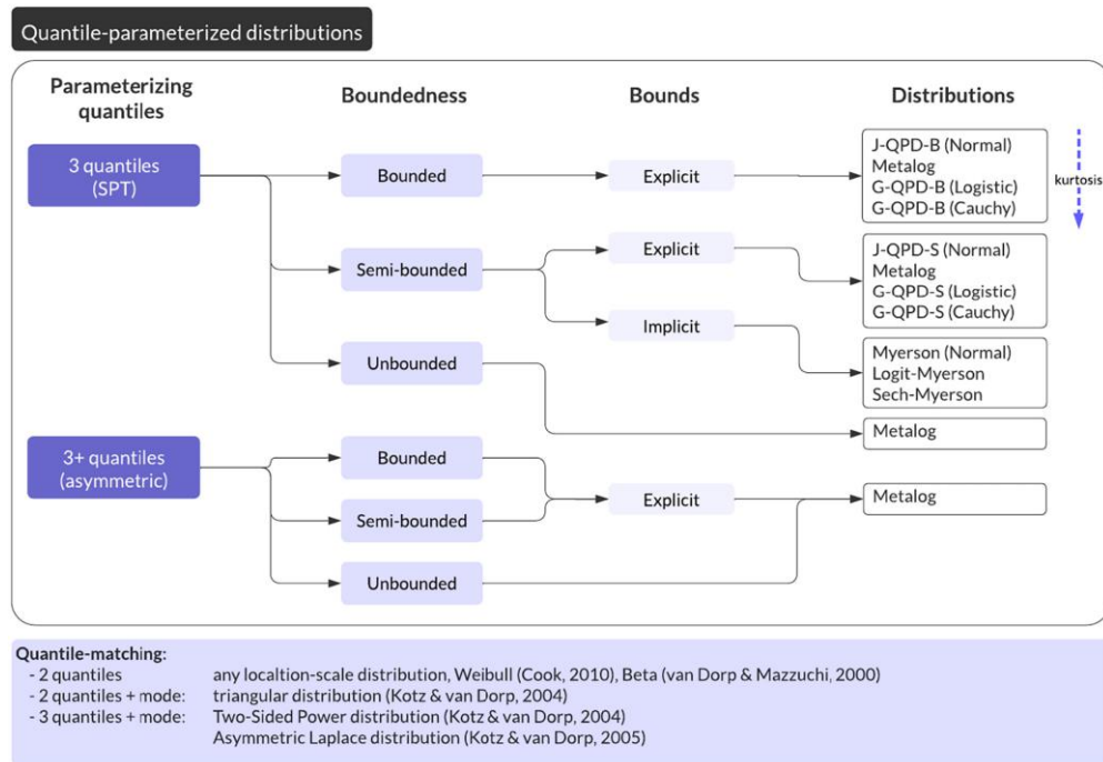
Figure 8. (Color online) Concept Map for Choosing Quantile-Parameterized Distribution
