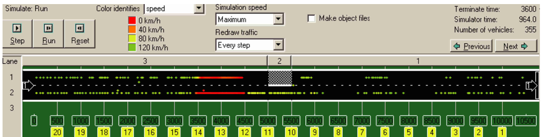
FIGURE 10. Screenshot of freeway stretch with a temporary bottleneck (e.g., an incident) coded in microsimulation model FOSIM (Vermijs and Schuurman [55]).
