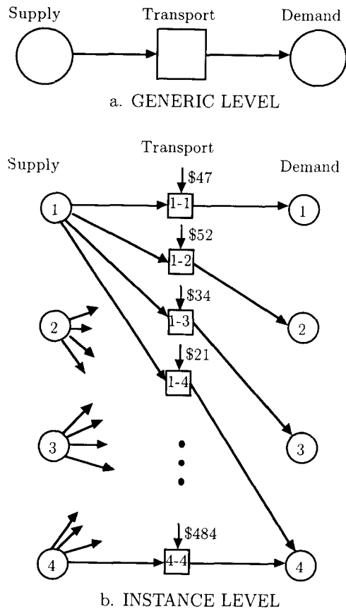
Figure 9. Activity-constraint diagrams for the transportation problem. In (a), the activity-constraint diagram for the generic transportation problem is shown. In (b), the activity-constraint diagram for a four-source, four-sink transportation problem instance is shown. Decision variables are represented by squares, and constraints are represented by circles. Note that for clarity in (b), many of the nodes and arcs are omitted.
