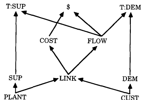
Figure 12. Structured modeling genus graph for the transportation problem. Compare this graph to the textual representation of SML in Figure 5. Each node represents a collection of elements in the model. Each arc a \rightarrow b indicates that genus b is defined, at least in part, by genus a . In short, the genus graph illustrates the interrelationships among genera.
