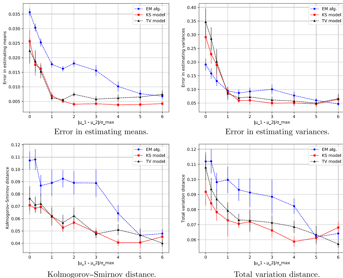
Figure 4. Performance as a Function of Separation \frac{|\mu_1 - \mu_2|}{\sigma_{\max}} Between the Gaussian Components for a One-Dimensional Gaussian Mixture with K = 2 Components and Training Sample Size n = 500
