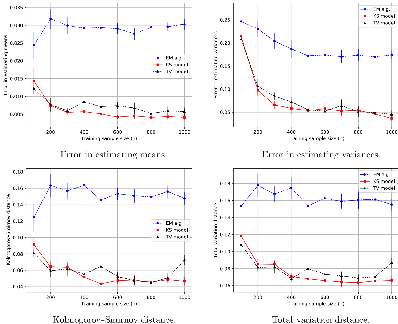
Figure 3. Performance as a Function of n for a One-Dimensional Gaussian Mixture with K = 2 Components and Separation |\mu_1 - \mu_2| = 1 \sigma_{\max}
