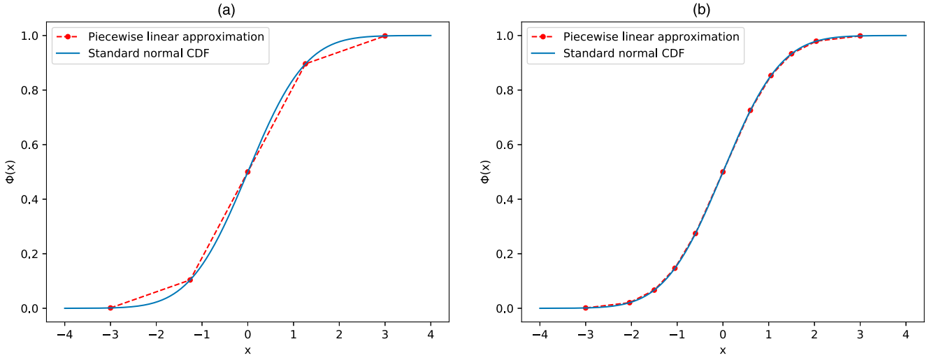
Figure 1. Optimal Piecewise Linear Approximations for the Standard Normal CDF
