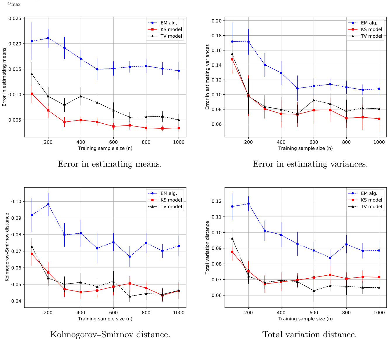
Figure 2. Performance as a Function of n for a One-Dimensional Gaussian Mixture with K = 2 Components and Separation |\mu_1 - \mu_2| = 2
