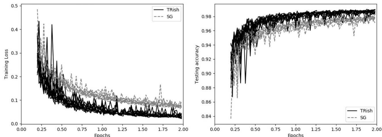
Figure 6. Average Training Loss and Testing Accuracy During the First Two Epochs when TRish and the SG Method Are Employed to Train a Convolutional Neural Network Using the mnist Data Set
