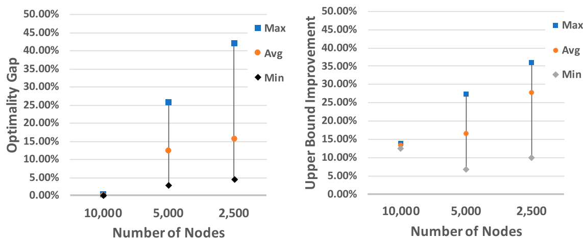
Figure 10. (Color online) Average Optimality Gaps (%) and Improvement (%) over the Shakarian Heuristic for BIP-Full on Large Simulated Graphs
