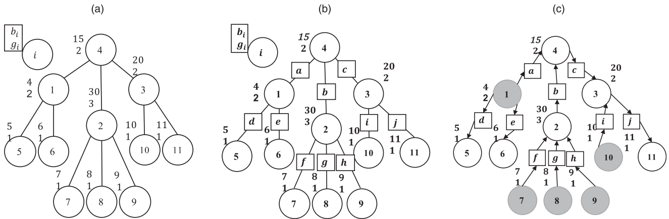
Figure 2. (a) WTSS Problem Instance, (b) G^t , and (c) A Valid Solution to BIP_{tree}
