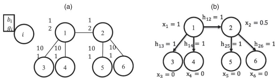
Figure 1. (a) WTSS Problem Instance and (b) Fractional Optimal Solution to ACK
