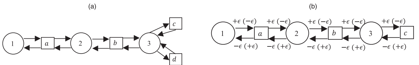
Figure 4. Illustrating the Proof of Theorem 1
