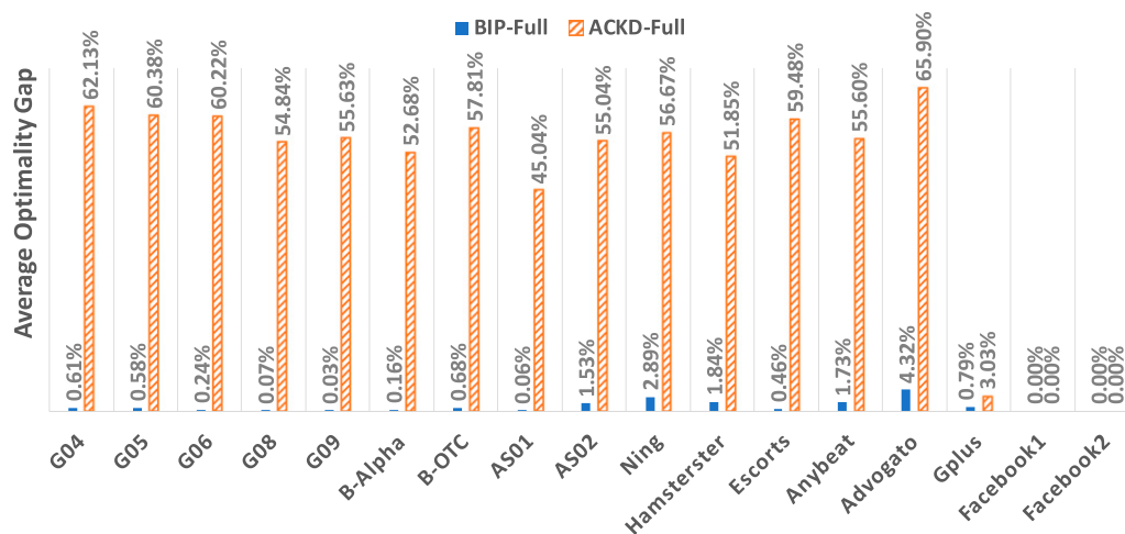
Figure 6. (Color online) Average Optimality Gap (%) of BIP-Full and ACKD-Full
