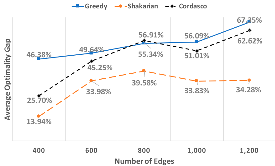
Figure 9. (Color online) Average Optimality Gaps (%) for the Greedy, Shakarian, and Cordasco Heuristic on Small (200 Node) Simulated Graphs
