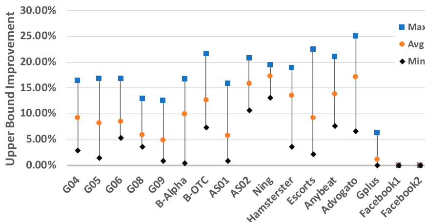
Figure 7. (Color online) Improvement (%) in BIP-Full Upper Bound over ACKD-Full Upper Bound on Real-World Graphs
