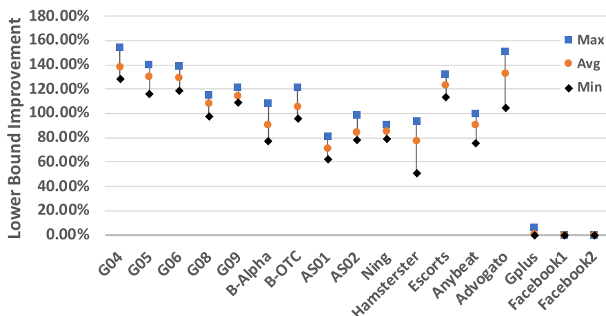
Figure 8. (Color online) Improvement (%) in BIP-Full Lower Bound over ACKD-Full Lower Bound on Real-World Graphs
