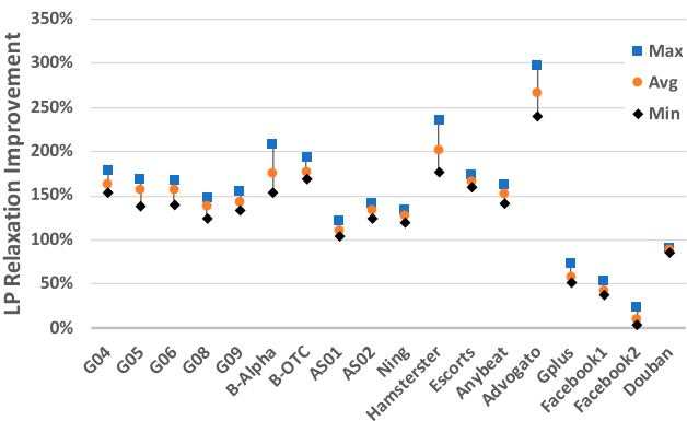
Figure 5. (Color online) Improvement (%) of the LP Relaxation of BIP over That of ACKD on Real-World Graphs
