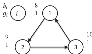
Figure 3. The Problem with Influence Propagation Around a Cycle
