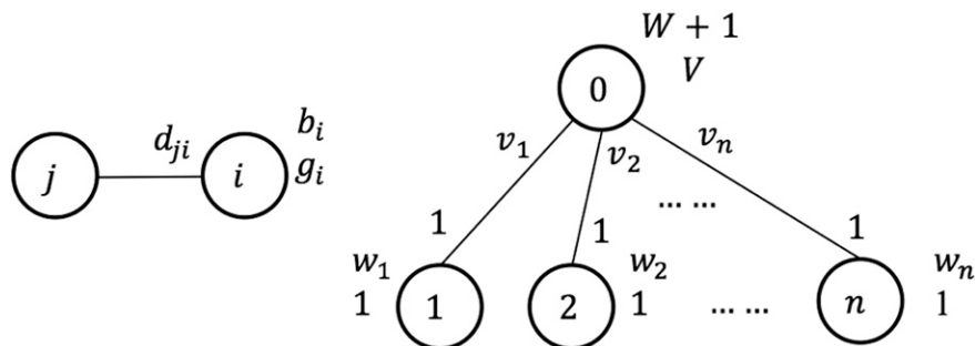
Figure A.1. Transforming a 0-1 Knapsack Problem to the WTSS Problem with Unequal Influence on Stars
