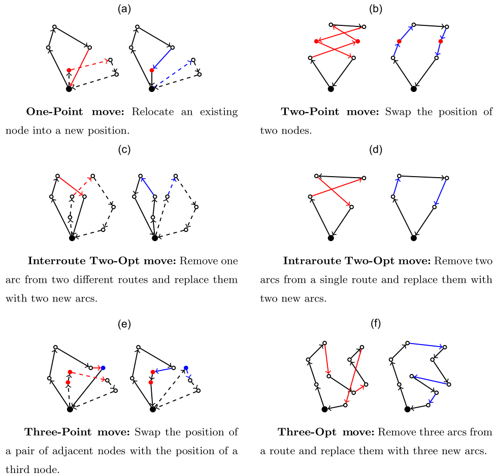
Figure 1. (Color online) Local Search Operators
