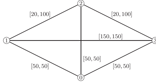
Figure 2. Graph with Budgeted Uncertainty Used in Example 1. The Node 0 is the Depot Node. The intervals contain all possible costs for an edge and \Gamma is set to 1.
