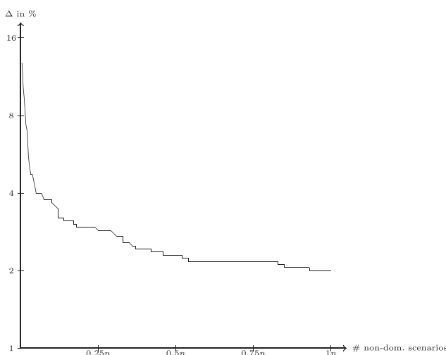
Figure 5. Percentage Difference Between the Heuristic Value and the Optimal Value in Terms of the Number of Generated Nondominated Scenarios, for a Budgeted Instance of P-n16-k8 with \Gamma = 15
