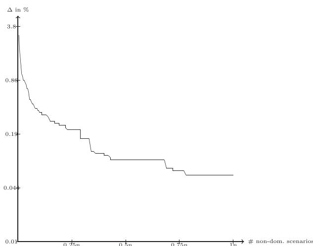
Figure 4. Percentage Difference Between the Heuristic Value and the Optimal Value in Terms of the Number of Generated Nondominated Scenarios, for an Ellipsoidal Instance of P-n16-k8 with \alpha = 0.95
