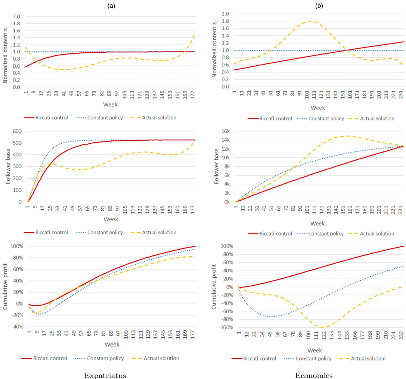
Figure 4. (Color online) Normalized Content Decisions (Top Figures), Follower-Base Trajectories (Middle Figures), and the Corresponding Cumulative Profits (Bottom Figures) for the Actual Solution, Riccati Control, and Constant Policy
