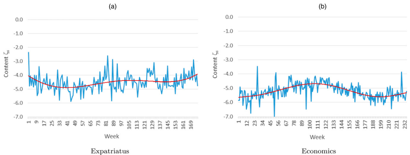
Figure 3. (Color online) Variation in \zeta_s Across Posts for Two of the Blogs
