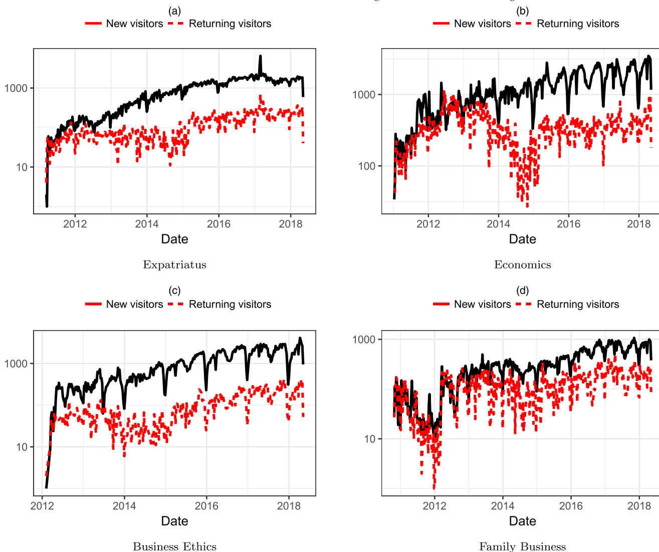
Figure 2. (Color online) Total Visits Per Week for New and Returning Visitors to the Four Blogs
