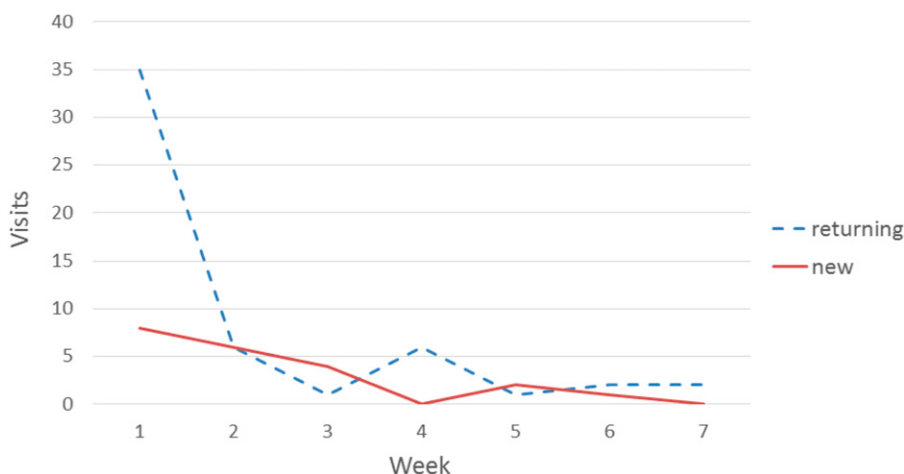
Figure 1. (Color online) Traffic Decay for a Single Post
