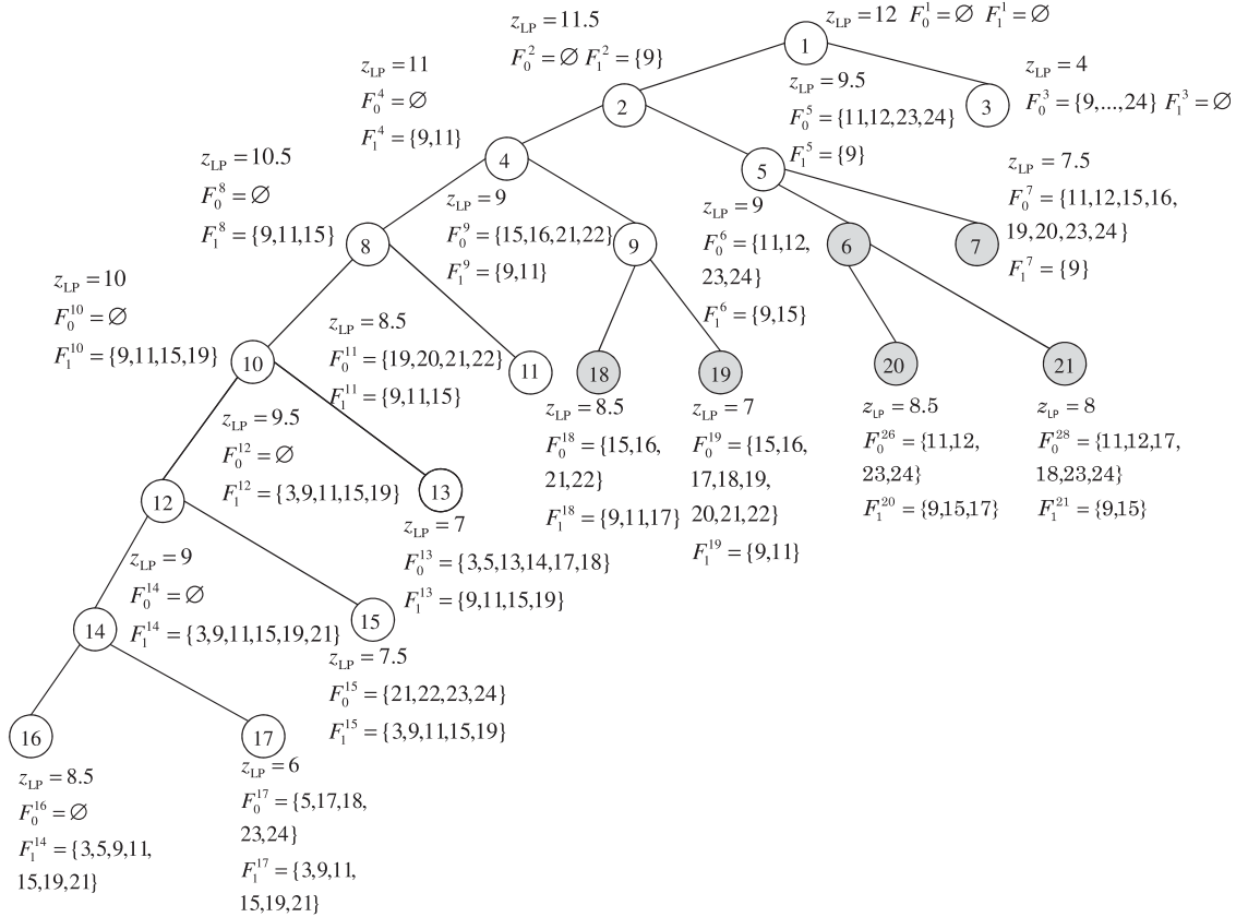
Figure 2. Search Tree by Orbital Branching
