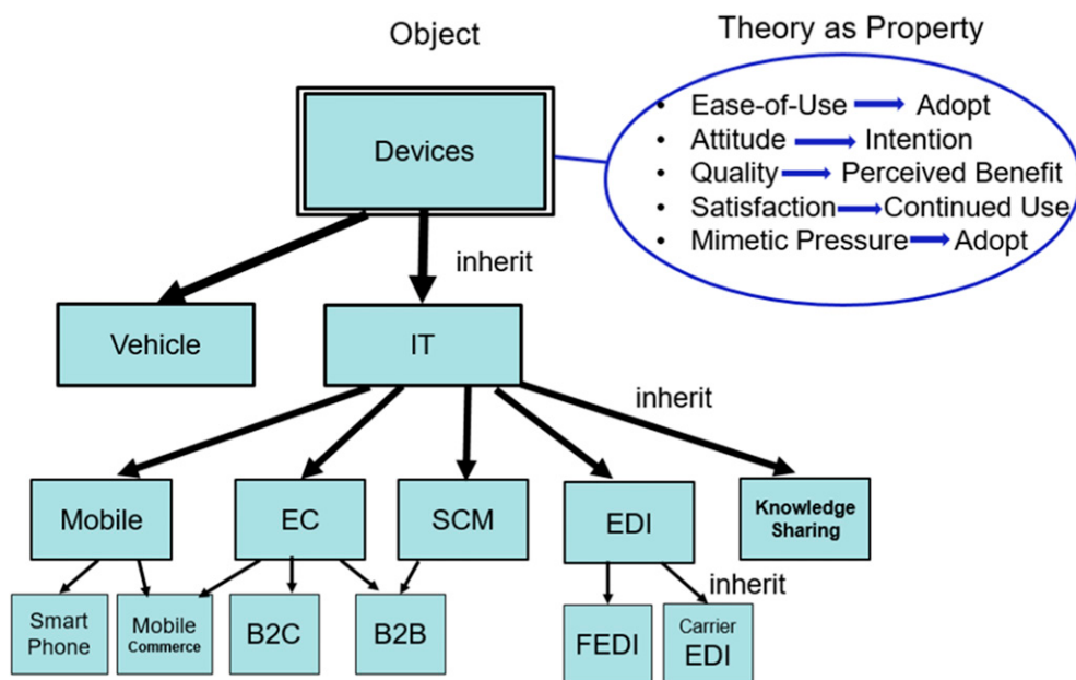
Figure 3. (Color online) Nature of Inherited Axiomatic Theories
