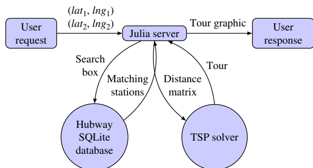
Figure 6 Design of the TSP Web Service That Students Implemented During the Capstone Project Modules
