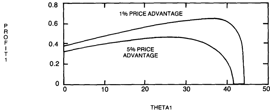
FIGURE 4. Plot of Profit (of I.ROBOT) as a Function of Its Position ( \Theta_1 ) with ROCON Fixed at \Theta_1 = 45^\circ and with a Price Advantage to ROCON ( p_2 < p_1 ).
