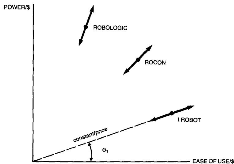
FIGURE 5. Price Equilibria: When Relative Positions ( \theta_1 ) Are Fixed Firms Can Adjust Prices. Movement in per-dollar space is indicated by heavy arrows.
