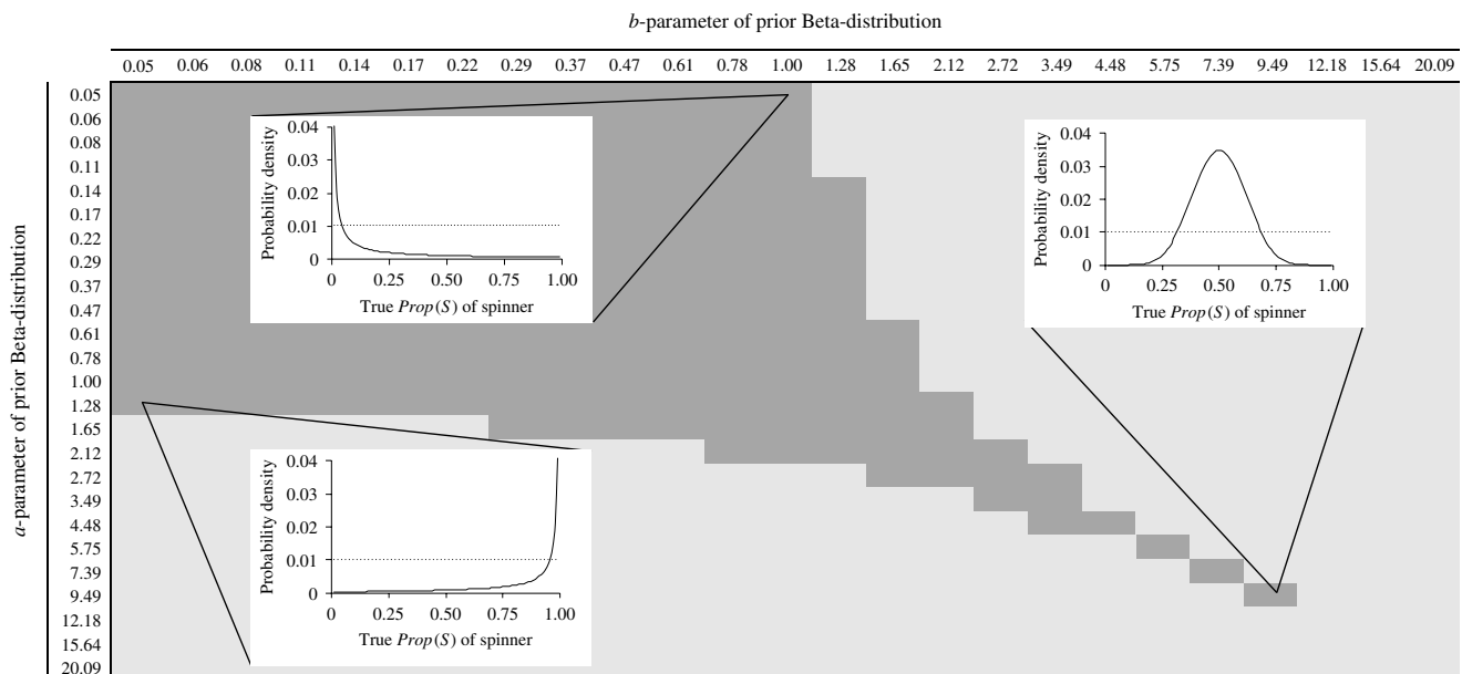
Figure 3. Range of a and b Parameters of a Beta _{(a,b)} -Distribution
