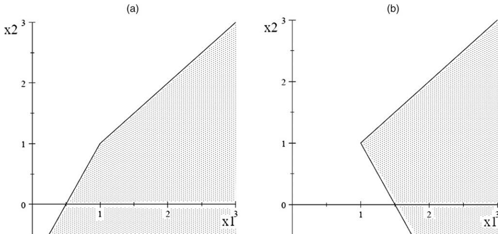
Figure 1. Bonus Regions for Correlation Coefficients 0.5 (Panel A) and −0.5 (Panel B)
