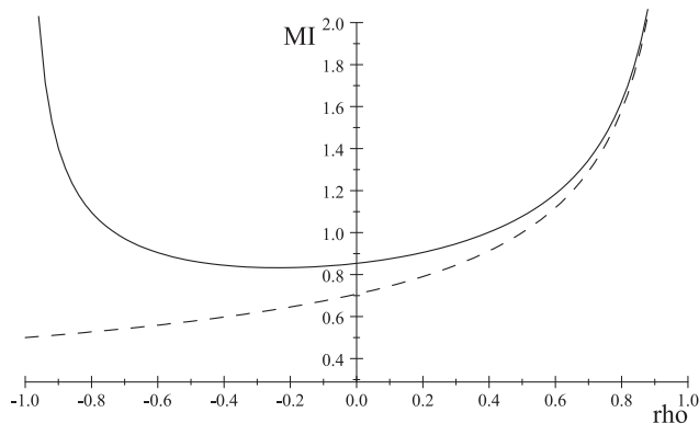
Figure 2. MIs as Functions of \rho
