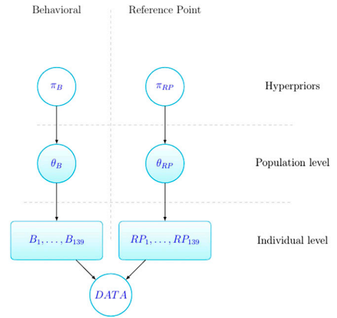
Figure 2. (Color online) Graphical Representation of Our Model
