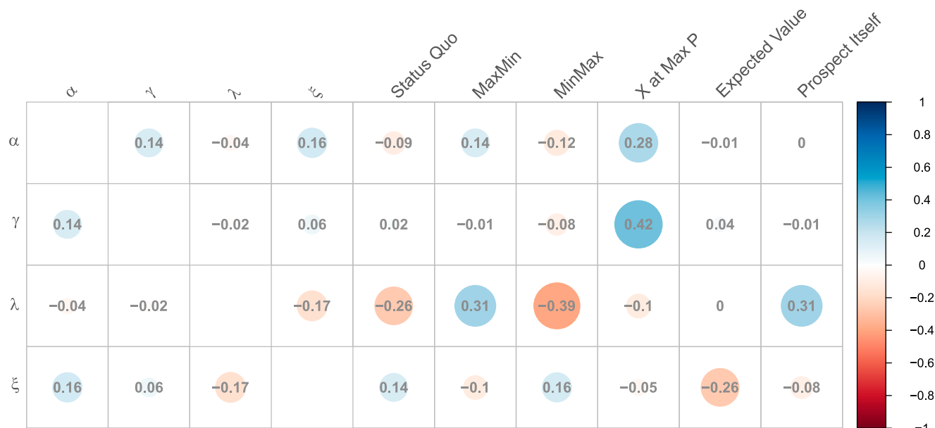
Figure 9. (Color online) Correlations Between Behavioral Parameters and Estimated Reference Point Rules
