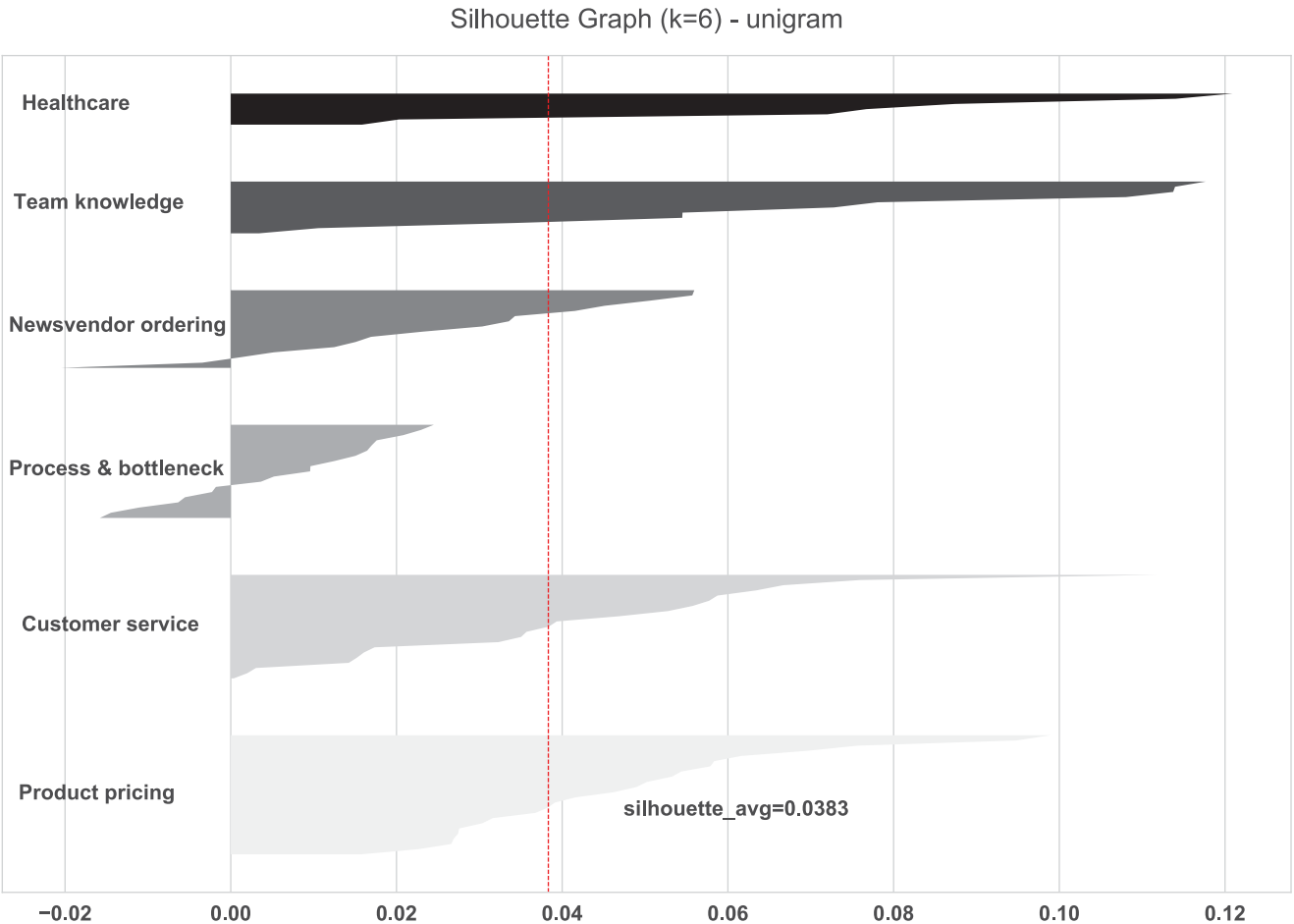
Figure A.1. (Color online) Silhouette of the Six Clusters Obtained with the NMF Algorithm
