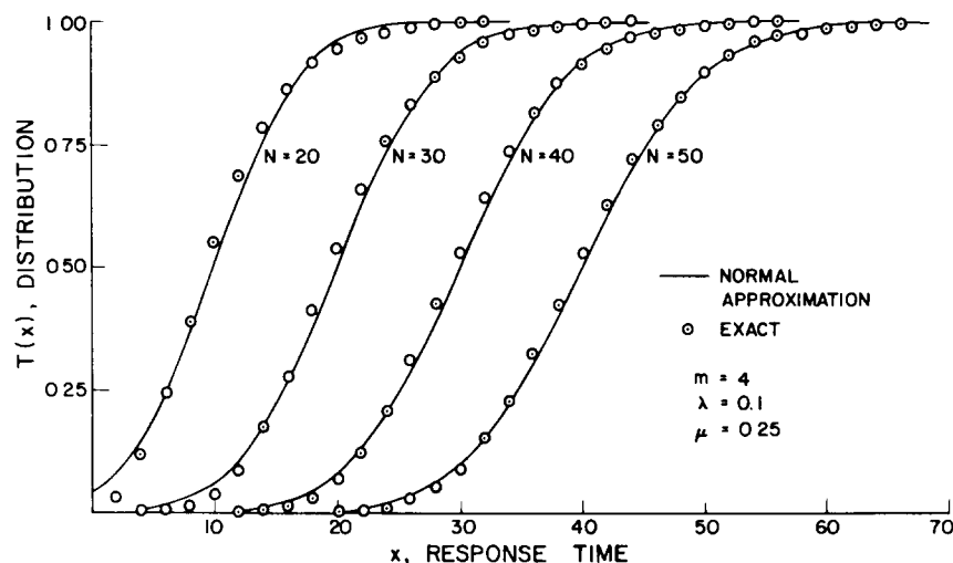
Figure 5. Response time distribution.
