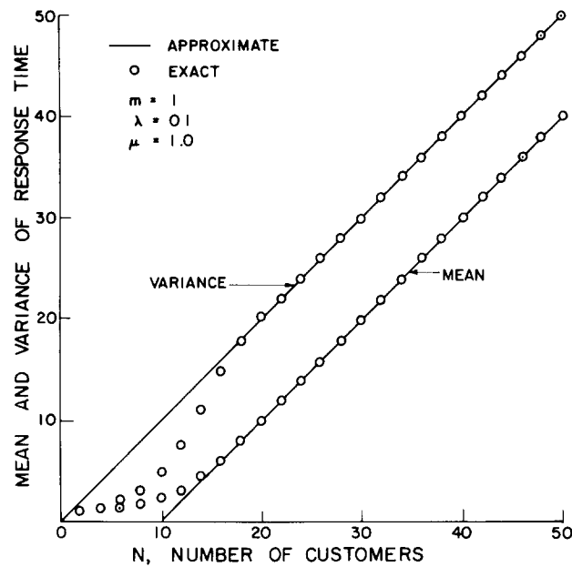
Figure 2. Mean and variance of response time vs. N .
