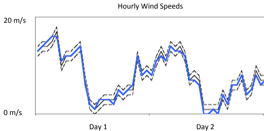
Figure 3 Two Days of Simulated Hourly Wind Speeds
