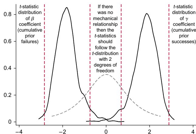
Figure 3. (Color online) Distribution of t -Statistics on Failure and Success Coefficients from 1,000 Randomly Drawn Data Sets
