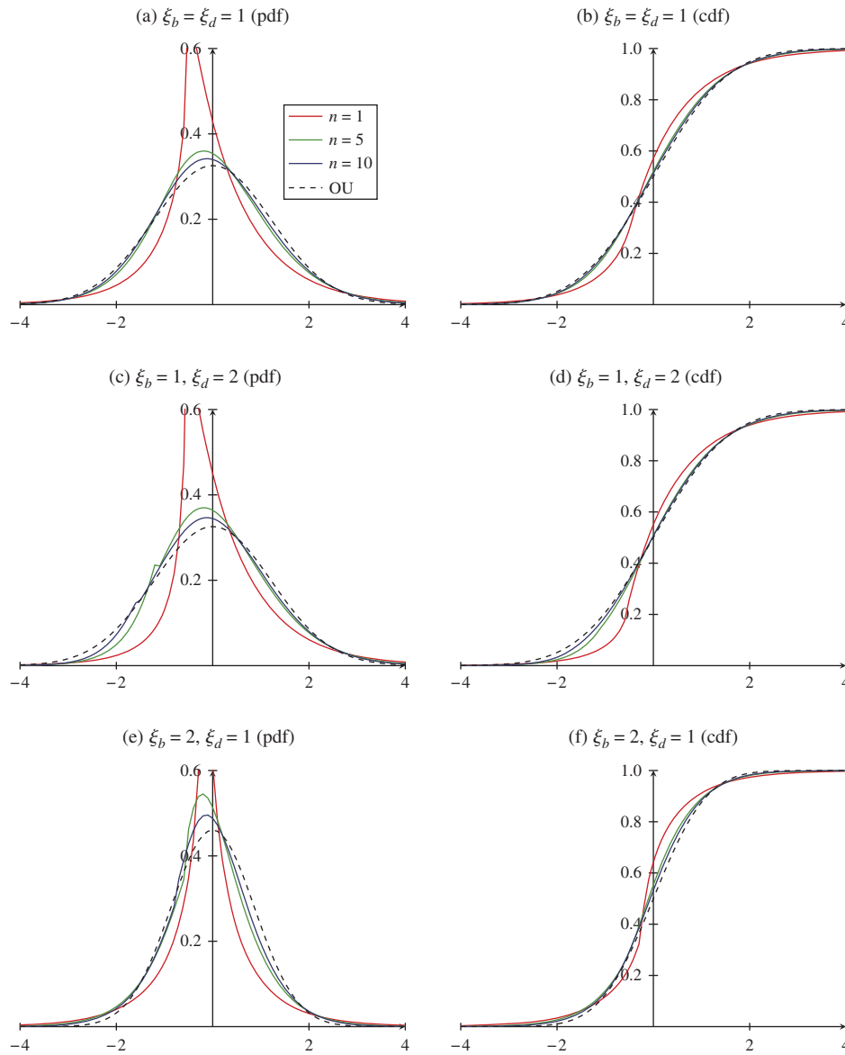
Figure 6. Steady-state density (left) and distribution (right) function of the normalized inventory process \hat{X}_n for n = 1, 5 and 10 with \lambda_b = 1 , \lambda_d = 0.5 and \mu_b = \mu_d = 1 , and of the OU process.
