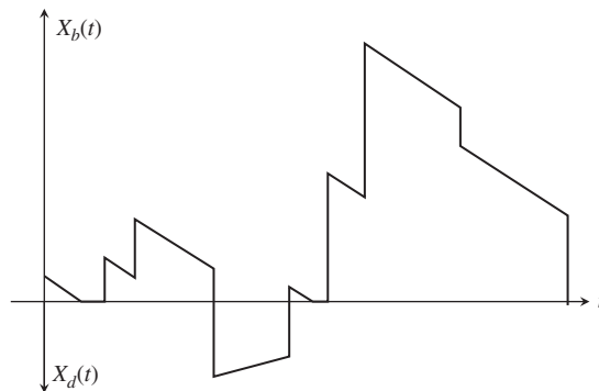
Figure 3. Sample path of the net amount of blood present if \xi_b = \xi_d = 0 .
