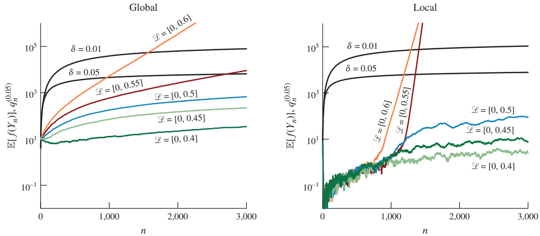
Figure 2. (Color online) Estimated mean curves of f(Y) when \mathcal{L} = [0, 0.4] , [0, 0.45] , [0, 0.5] , [0, 0.55] , or [0, 0.6] for a simple queue compared to estimated q^{(0.05)} curves with \delta = 0.01 or \delta = 0.05 .
