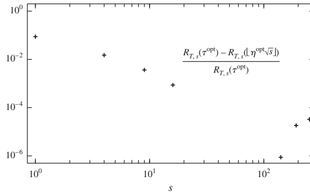
Figure 4. The relative error (R_{T,s}(\tau^{\text{opt}}) - R_{T,s}(\lfloor \eta^{\text{opt}} \sqrt{s} \rfloor)) / R_{T,s}(\tau^{\text{opt}}) as a function of s . The missing points indicate an error that is strictly zero. The errors that are non-zero arise due to the QED approximation for the optimal admission threshold being off by just one state.
