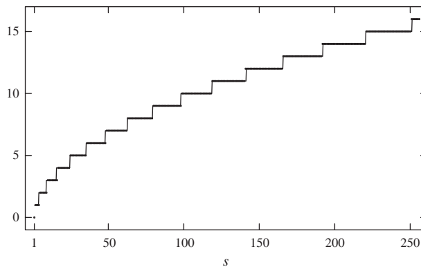
Figure 3. The true optimal admission threshold \tau^{\text{opt}} as a function of s , together with the (almost indistinguishable) QED approximation \lfloor \eta^{\text{opt}} \sqrt{s} \rfloor .
