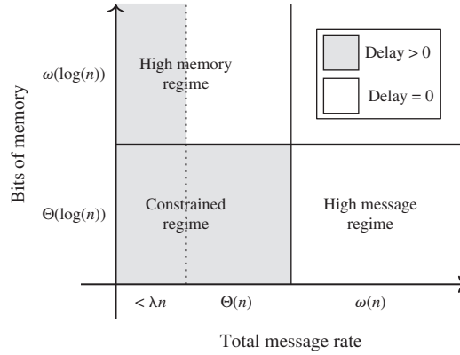
Figure 3. Resource requirements of the three regimes, and the resulting asymptotic delays.
