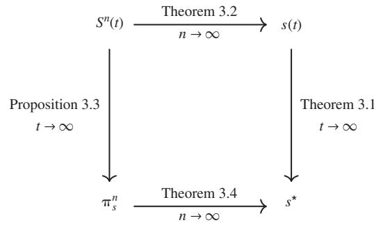
Figure 4. Relationship between the stochastic system and the fluid model.
