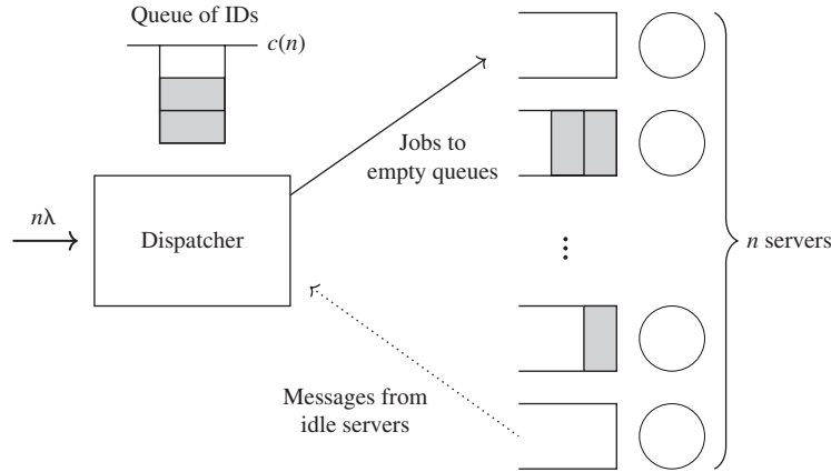
Figure 2. Resource constrained pull-based policy. Jobs are sent to queues associated with idle servers, based on tokens in the virtual queue. If no tokens are present, a queue is chosen at random.
