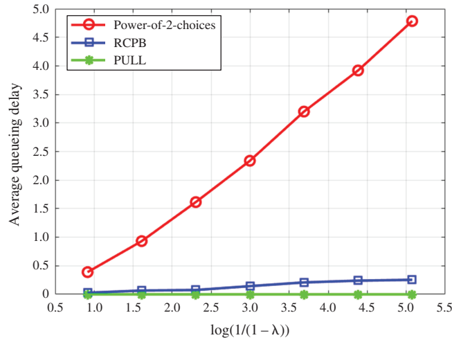
Figure 5. Average delay of the power-of-2-choices policy (red circles) vs. our policy (blue squares) vs. PULL (green asterisks).
