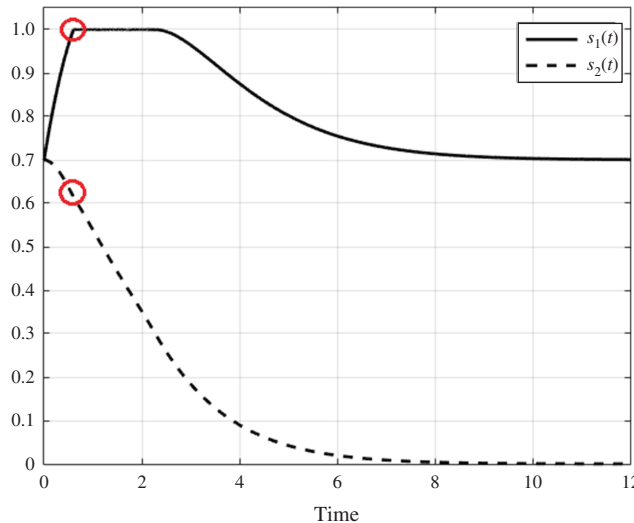
Figure 6. An example of a non-differentiable solution for the high message regime, with \lambda = 0.9 , s_1(0) = s_2(0) = s_3(0) = 0.7 , and s_i(0) = 0 for all i \geq 4 .
