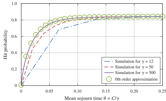
Figure 4. Convergence of the hit probability curves obtained in the experiments to the 0th order Che approximation.
