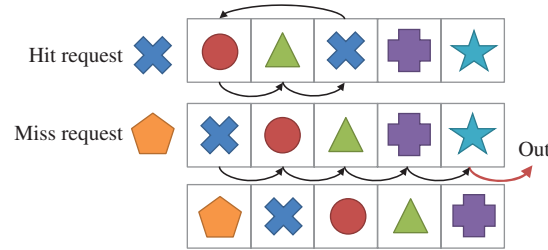
Figure 1. The LRU eviction policy handling a hit and a miss request on a cache of size C = 5 .
