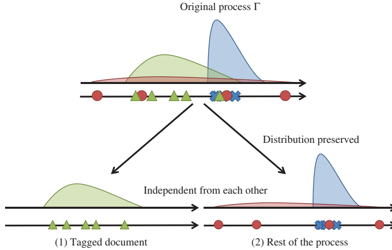
Figure 3. Illustration of request process \xi under the averaged Palm distribution. The original process is decomposed into: (1) the tagged document and (2) the rest of the process. These are mutually independent, and the rest of the process has the same distribution as the original process.
