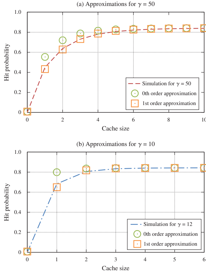
Figure 5. Comparison between hit probability curves obtained in the experiments and their analytic approximations in the case of low \gamma .
