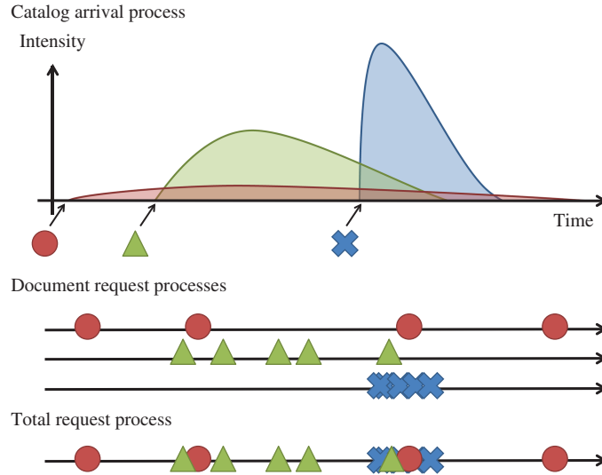
Figure 2. A Sample of the document arrival and request processes. Top: Each catalog arrival triggers a function representing the request intensity for the corresponding document. Bottom: A sample of the document request processes. Their superposition generates the total request process.
