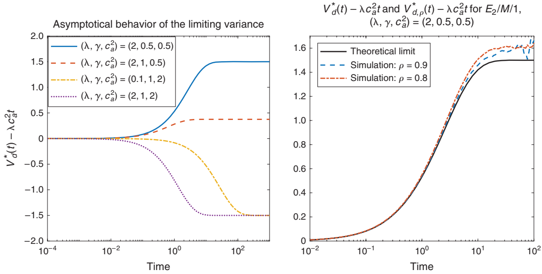
Figure 1. On the left is V_d^*(t) - \lambda c_a^2 t for four sets of parameters calculated from numerically inverting (31). On the right is the HT-scaled and centered variance V_{d,\rho}^*(t) - \lambda c_a^2 t for \rho = 0.8 and 0.9 in the E_2/M/1 model with \lambda = 2 , estimated by simulation, compared with the theoretical limit V_d^*(t) - \lambda c_a^2 t .
