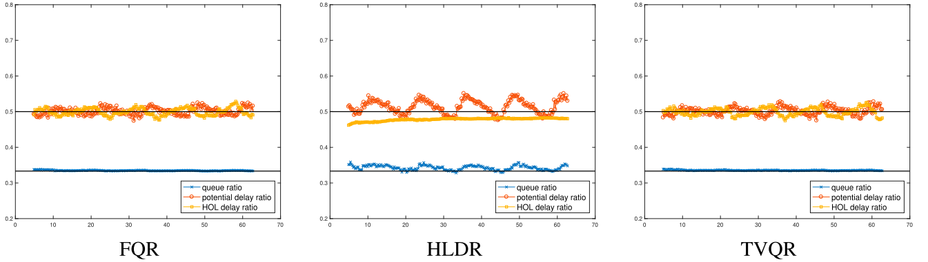
Figure 3. (Color online) Queue and Delay Ratios for a Two-Class M_t/M/s_t Queue with Arrival-Rate Functions \lambda_1(t) = 60 + 20 \sin(t/2) , \lambda_2 = 90 + 30 \sin(t/2) , Common Service Rate \mu = 1 , Without Abandonment ( \theta_1 = \theta_2 = 0 ), and \tilde{c} = 0.25
