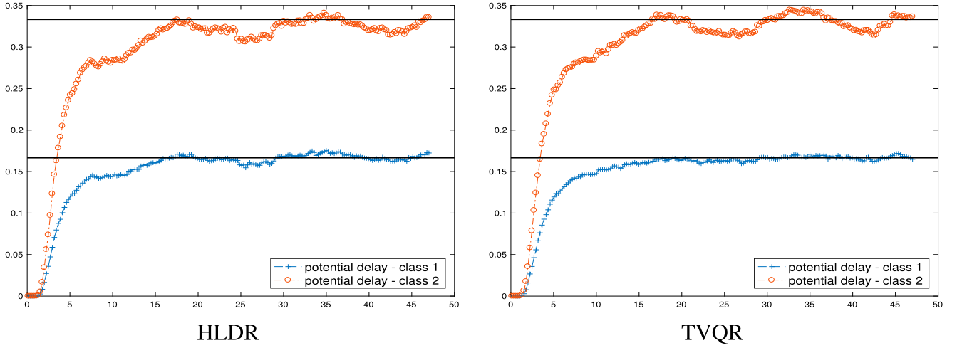
Figure 8. (Color online) Estimated Expected Potential Delays for a Two-Class M_t/G/s_t + M Queue with Arrival-Rate Functions \lambda_1(t) = 60 - 20 \sin(2t/5) , \lambda_2 = 90 + 30 \sin(2t/5) , and Abandonment Rate \theta = 1
