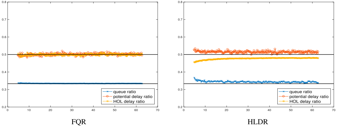
Figure 1. (Color online) Queue and Delay Ratios for a Two-Class Stationary M/M/s Queue with Arrival Rate Functions \lambda_1 = 60 , \lambda_2 = 90 , Common Service Rate \mu = 1 , Without Abandonment ( \theta_1 = \theta_2 = 0 ), and \tilde{c} = 0.25
