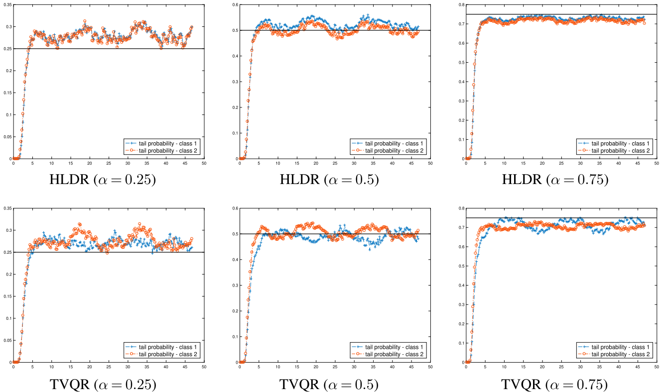
Figure 7. (Color online) Tail Probabilities for a Two-Class M_t/M/s_t + M Queue with Arrival-Rate Functions \lambda_1(t) = 60 - 20 \sin(2t/5) , \lambda_2 = 90 + 30 \sin(2t/5) , Common Service Rate \mu = 1 , Abandonment Rate \theta = 1 , and Minimum Staffing Function c^* Derived from (57)
