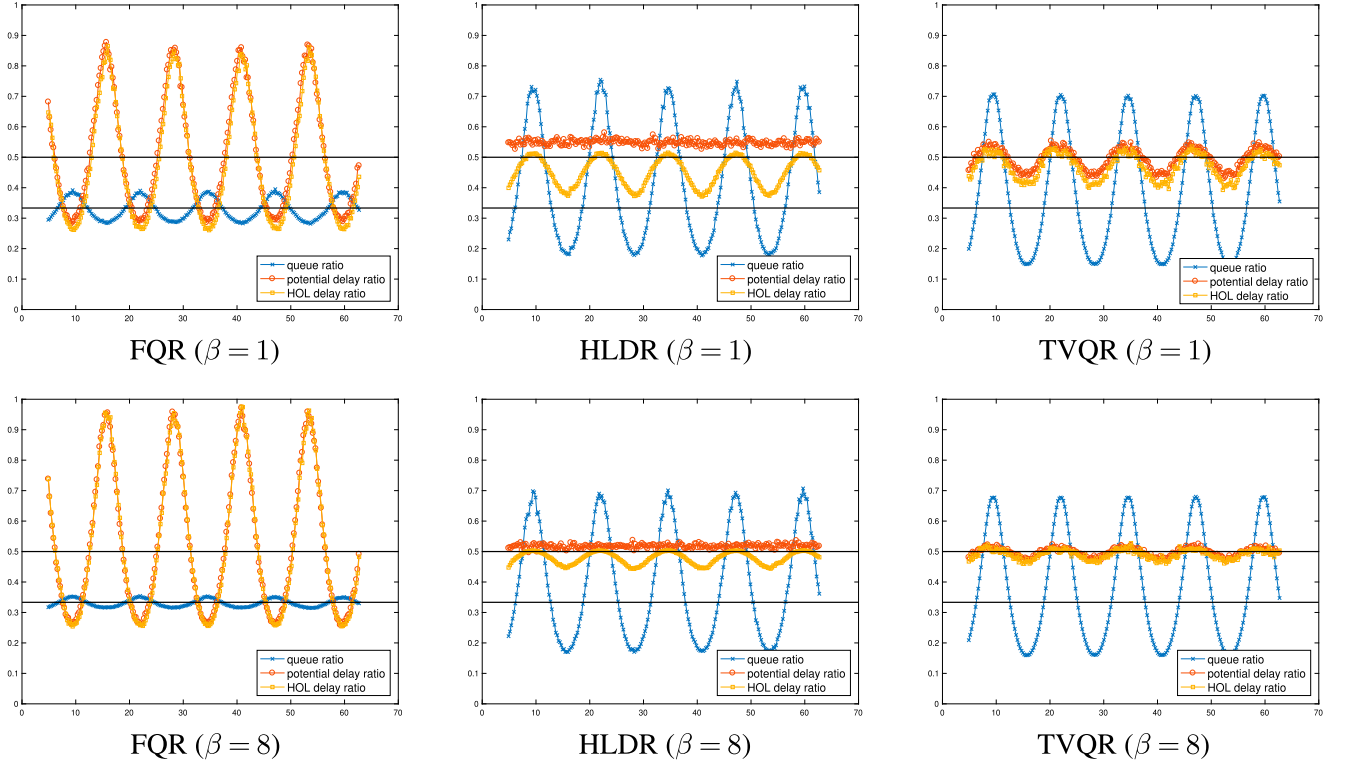
Figure 4. (Color online) Queue and Delay Ratios as a Function of System Size for a Two-Class M_t/M/s_t + M Queue with Arrival Rate Functions \lambda_1(t) = \beta \cdot (60 - 20 \sin(t/2)) , \lambda_2 = \beta \cdot (90 + 30 \sin(t/2)) , Service Rate \mu = 1 , Abandonment Rates \theta_1 = \theta_2 = 0.5 , and Safety Staffing Function c \equiv 0 : The Cases \beta = 1 and \beta = 8
