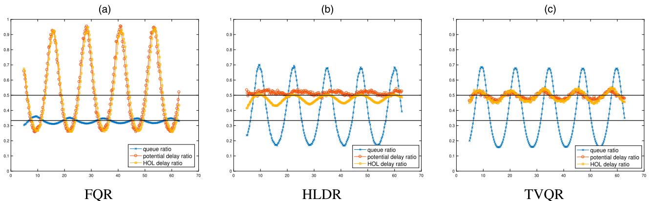
Figure 2. (Color online) Queue and Delay Ratios for a Two-Class M_t/M/s_t Queue with Arrival Rate Functions \lambda_1(t) = 60 - 20 \sin(t/2) , \lambda_2 = 90 + 30 \sin(t/2) , Common Service Rate \mu = 1 , Without Abandonment ( \theta_1 = \theta_2 = 0 ), and \tilde{c} = 0.25
