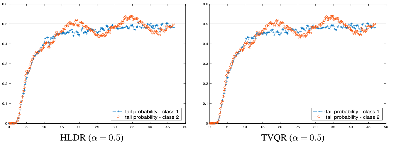
Figure 9. (Color online) Tail Probabilities for a Two-Class M_t/G/s_t + M Queue with Arrival-Rate Functions \lambda_1(t) = 60 - 20 \sin(2t/5) , \lambda_2 = 90 + 30 \sin(2t/5) , and Abandonment Rate \theta = 1
