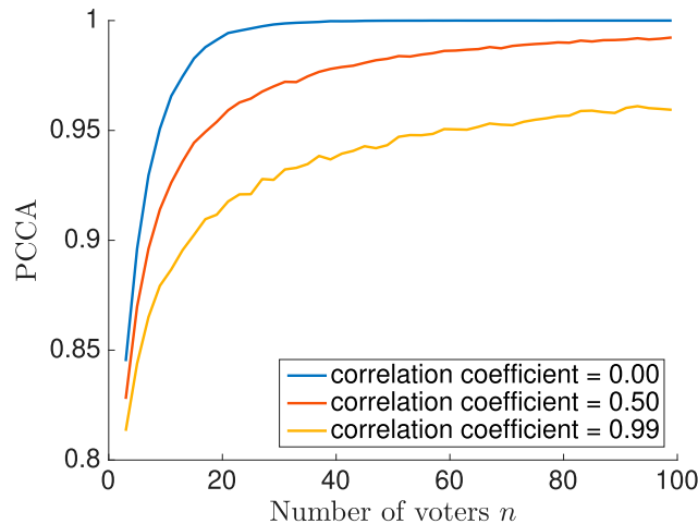
Figure 2. The PCCAs for Various Correlation Coefficients
