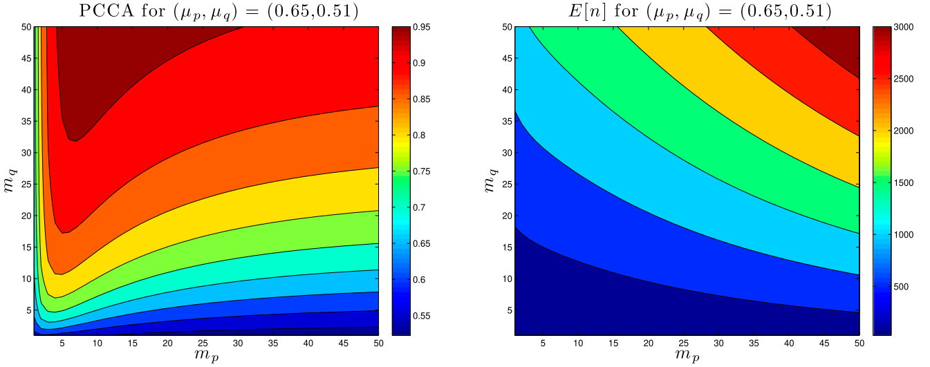
Figure 3. The PCCA (Left) and E[n] (Right) as a Function of m_p and m_q Under the Random Walk Model
