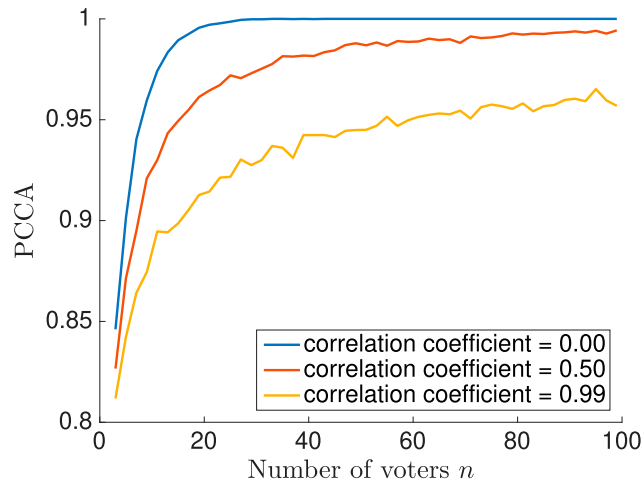
Figure 4. The PCCAs for Various Correlation Coefficients
