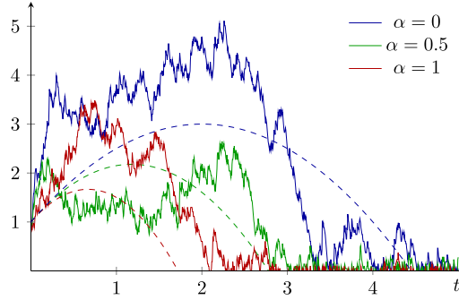
Figure 1. Sample Paths of the Process \mathbf{Q}_n(\cdot) for Various Values of \alpha and n = 10^4
