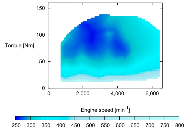
Figure 1. (Color online) Specific Fuel-Consumption Diagram Shows the Fuel Consumption in Grams per Kilowatt Hour
