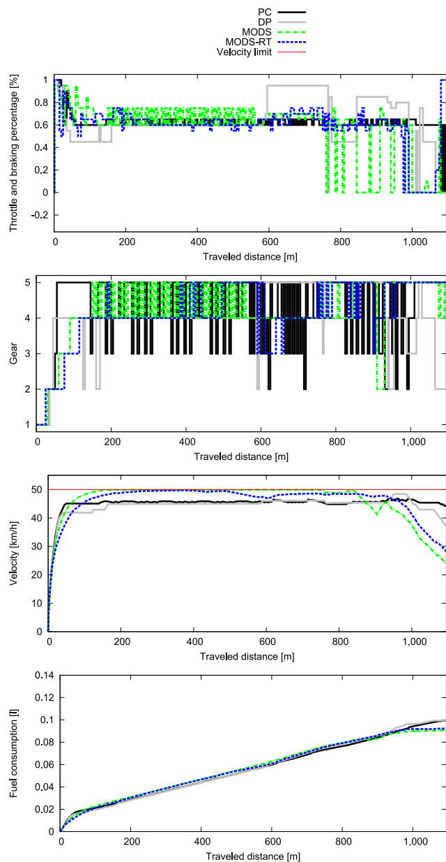
Figure 10. (Color online) Examples of Vehicle Behavior on the Second Route when Applying Driving Strategies with a Traveling Time of Around 1.5 Minutes
