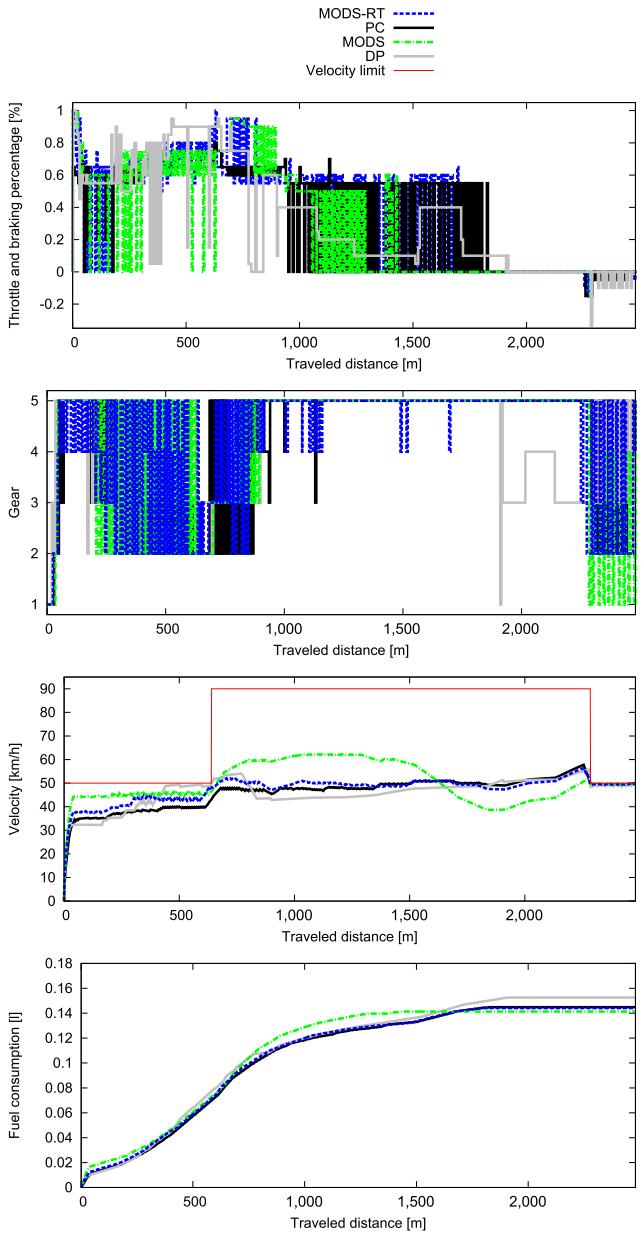
Figure 12. (Color online) Examples of Vehicle Behavior on the Third Route when Applying Driving Strategies with a Terminal Velocity of Around 50 Kilometers per Hour
