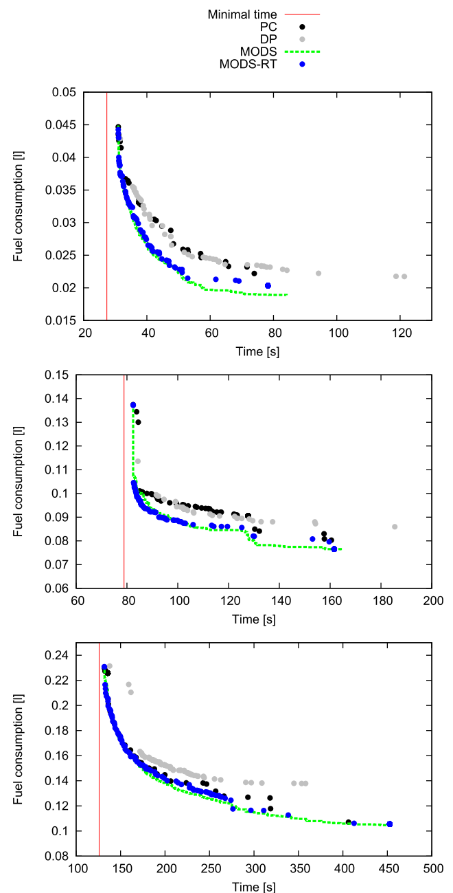
Figure 7. (Color online) Nondominated Driving Strategies in the Objective Space for the First Route (Top), Second Route (Middle), and Third Route (Bottom)
