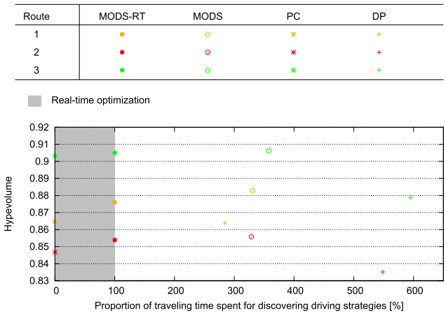
Figure 8. (Color online) Hypervolumes Obtained with the Algorithms with Respect to Proportion of Spent Time
