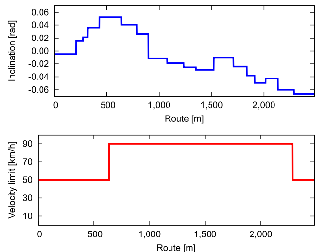
Figure 6. (Color online) Inclinations and Velocity Limits of the Third Testing Route
