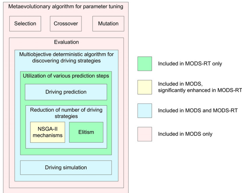
Figure 3. (Color online) A Schematic View of Differences Between MODS-RT and Its Predecessor, MODS
