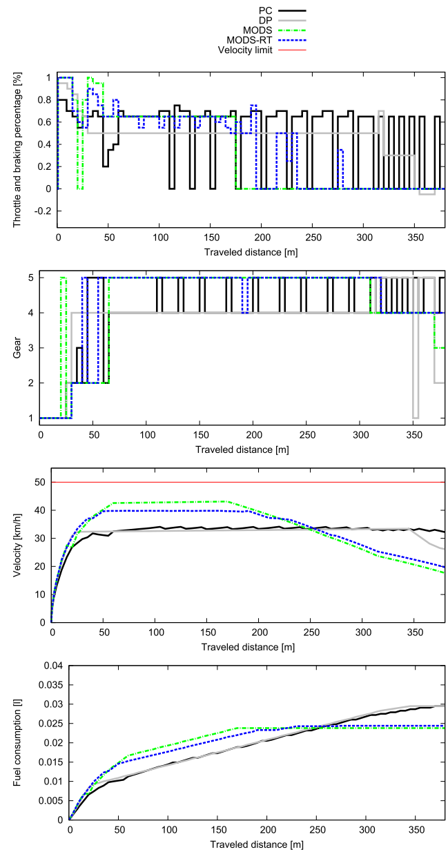
Figure 9. (Color online) Examples of Vehicle Behavior on the First Route when Applying Driving Strategies with a Traveling Time of Around 45 Seconds
