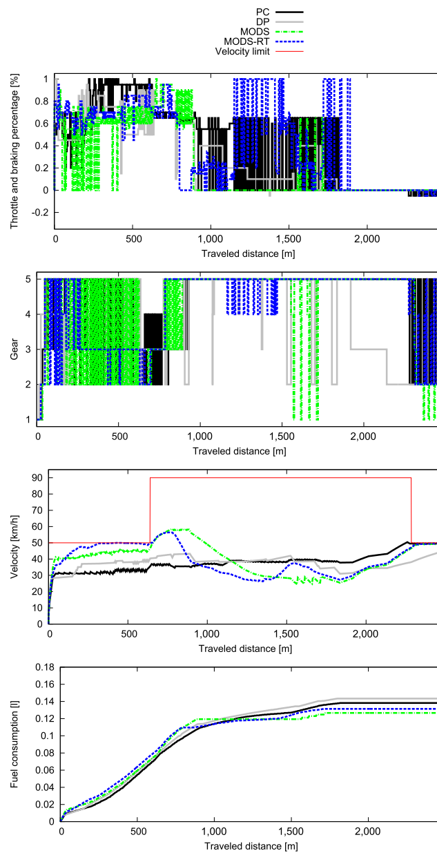
Figure 11. (Color online) Examples of Vehicle Behavior on the Third Route when Applying Driving Strategies with a Traveling Time of Around Four Minutes
