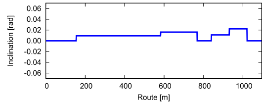
Figure 5. (Color online) Inclinations of the Second Testing Route
