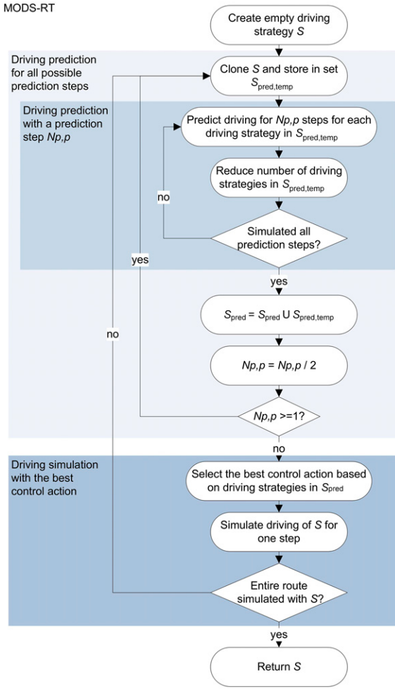
Figure 2. (Color online) A Schematic View of MODS-RT
